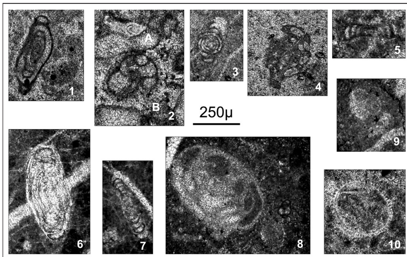
Text-Fig. 14. Foraminifera of the section in the ski trail between Gjaidalm and Krippenstein. 1 = Agathammina austroalpina KRISTAN-TOLLMANN & TOLLMANN, sample G 2; 2 = Fron-dicularia woodwardi HOWCHIN (A) and Trochammina almtalensis KOEHN-ZANINETTI (B), sample G 2; 3 = Glomospirella amplifata KRISTAN-TOLLMANN, sample G 3; 4 = Pilammina densa PANTIČ, sample G 2; 5 = Ammodiscus cf. incertus (D'ORBIGNY), sample G 3; 6 = Aulotortus sinuosus WEYNSCHENK, sample G 3; 7 = Angulodiscus tenuis KRISTAN, sample G 3; 8 = Angulodiscus friedli (KRISTAN-TOLLMANN), sample G 3; 9 = Oberhauserellidae sp., sample G 3; 10 = Radiolaria, sample G 3.
