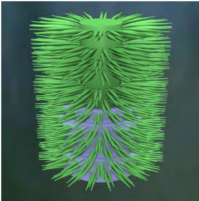
Text-Fig. 23. Reconstruction of Diplopore debilis (like Pl. VIII, Fig. 8), specimen with strongly thickened branches.
