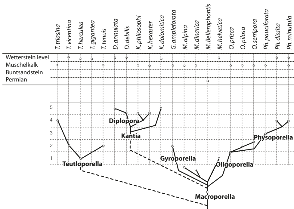
Text-Fig. 24. Tentative phyletic tree of the Diploporidae.
