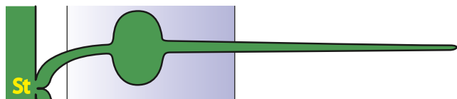
Text-Fig. 22. Longitudinal section through a branch of Diploporella annulata with a globular broadening (Sporangium?). St = main axis.
