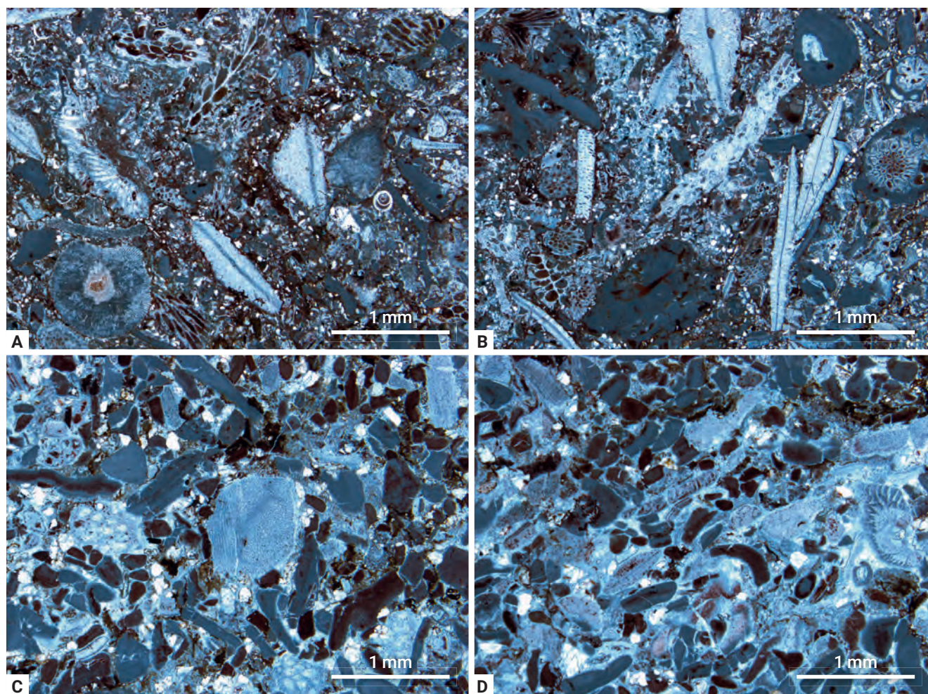
Text-Fig. 3. Thin-section images of Priabonian limestone from Kirchberg: A, B: Large, thin and disc-shaped Discocyclina sp. in association with coralline algal debris and bryozoans. C, D: coralline algae debris, orthophragminids and bryozoans.
