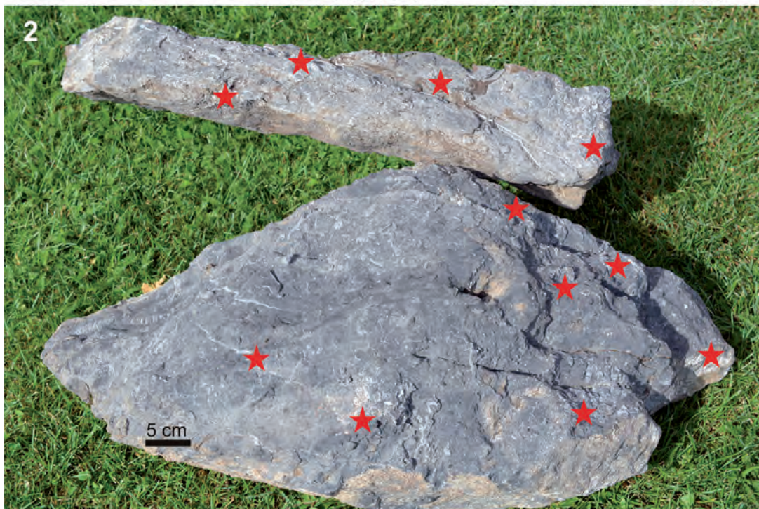
Text-Fig. 2. 1: Diagrams of the stratigraphical succession in the southern hillside of the Gail Valley indicating the location of the boulder (red star). 2: Picture of the boulder showing the location of some Lonsdaleia colonies (red stars).
