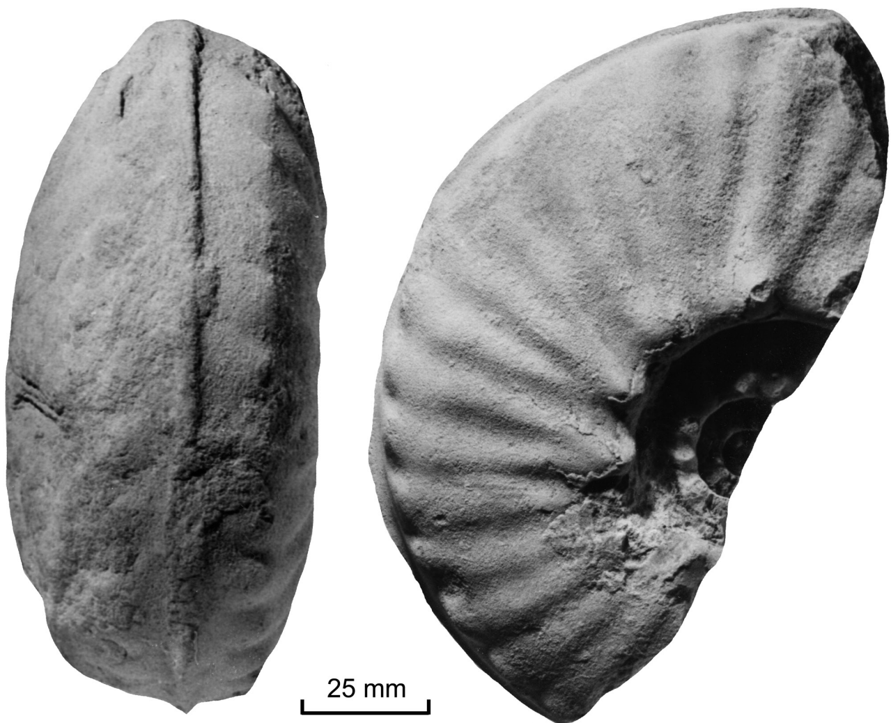
Text-Fig. 11. Pervinquieria ( Subschloenbachia ) sp., GBA 2016/003/0009, ex situ at the Mfamosing Quarry. Figures are x 1.
