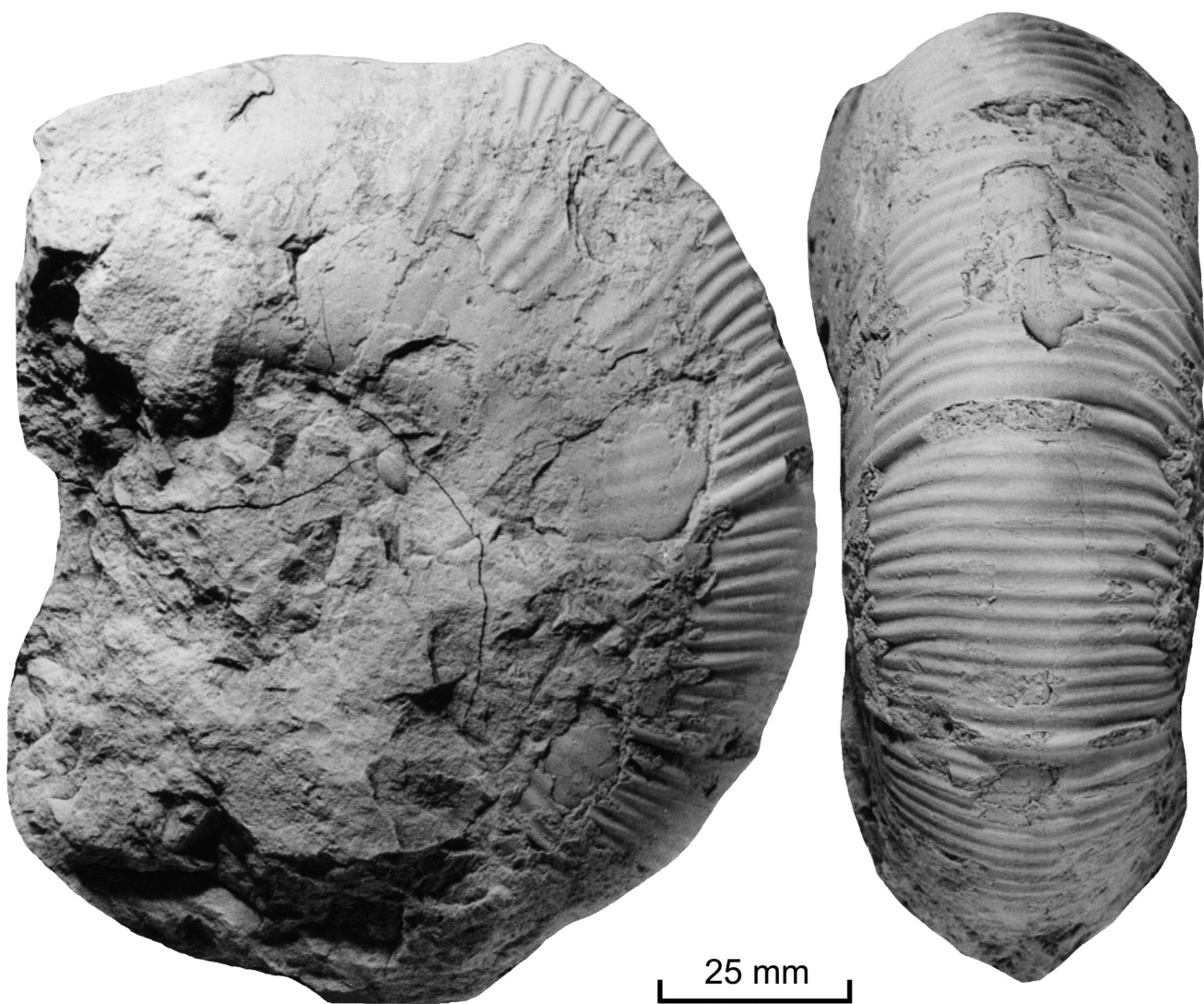
Text-Fig. 6. Puzosia (Anapuzosia) sp. GBA 2016/003/0019. Figures are x 1.
