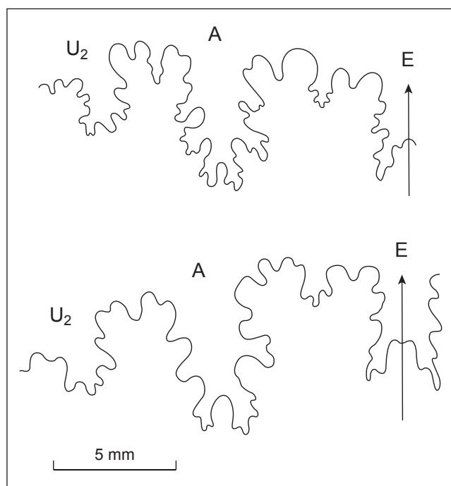
Text-Fig. 16. External sutures of Acompsoceras calabarensis ZABORSKI, 1985; A (top): GBA 2016/003/0052; B (bottom): GBA 2016/003/0051.
