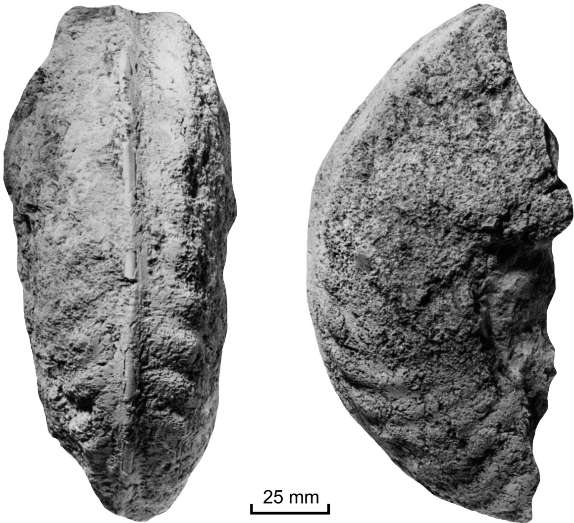
Text-Fig. 12. Arestoceras sp. GBA 2016/003/0008. Figures are x 1.
