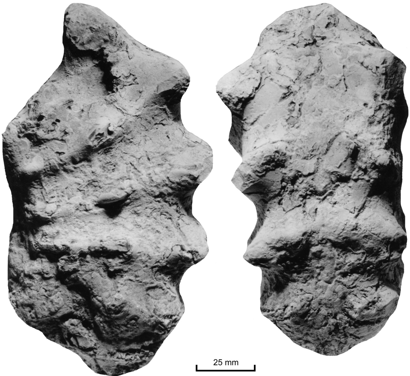
Text-Fig. 15. Sharpeiceras florencae SPATH, 1925. GBA 2016/003/0047, the Lower Cenomanian part of the Odukpani Formation at the 77/50 locality (Text-Fig. 1). Figures are natural size.
