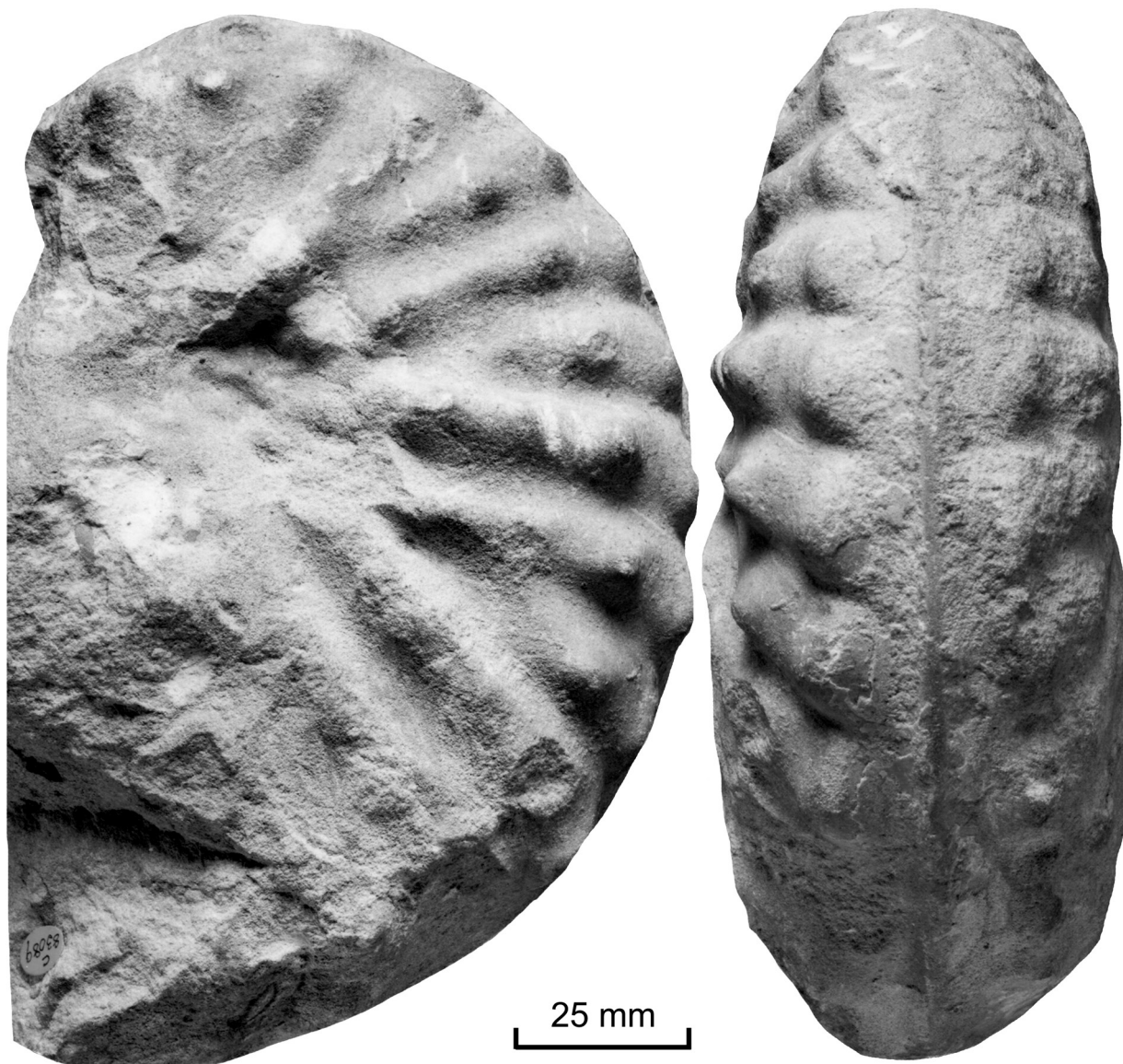
Text-Fig. 10. Pervinquieria (Subschloenbachia) cf. perinflata (SPATH, 1921), BMNH C83089, collected by P.M.P. Zaborski from “the top surface of the main limestone of the Upper Albian Mfamosing Formation at the Mfamosing Quarry”. Figures are x 1 (photos courtesy of the Natural History Museum, London).
