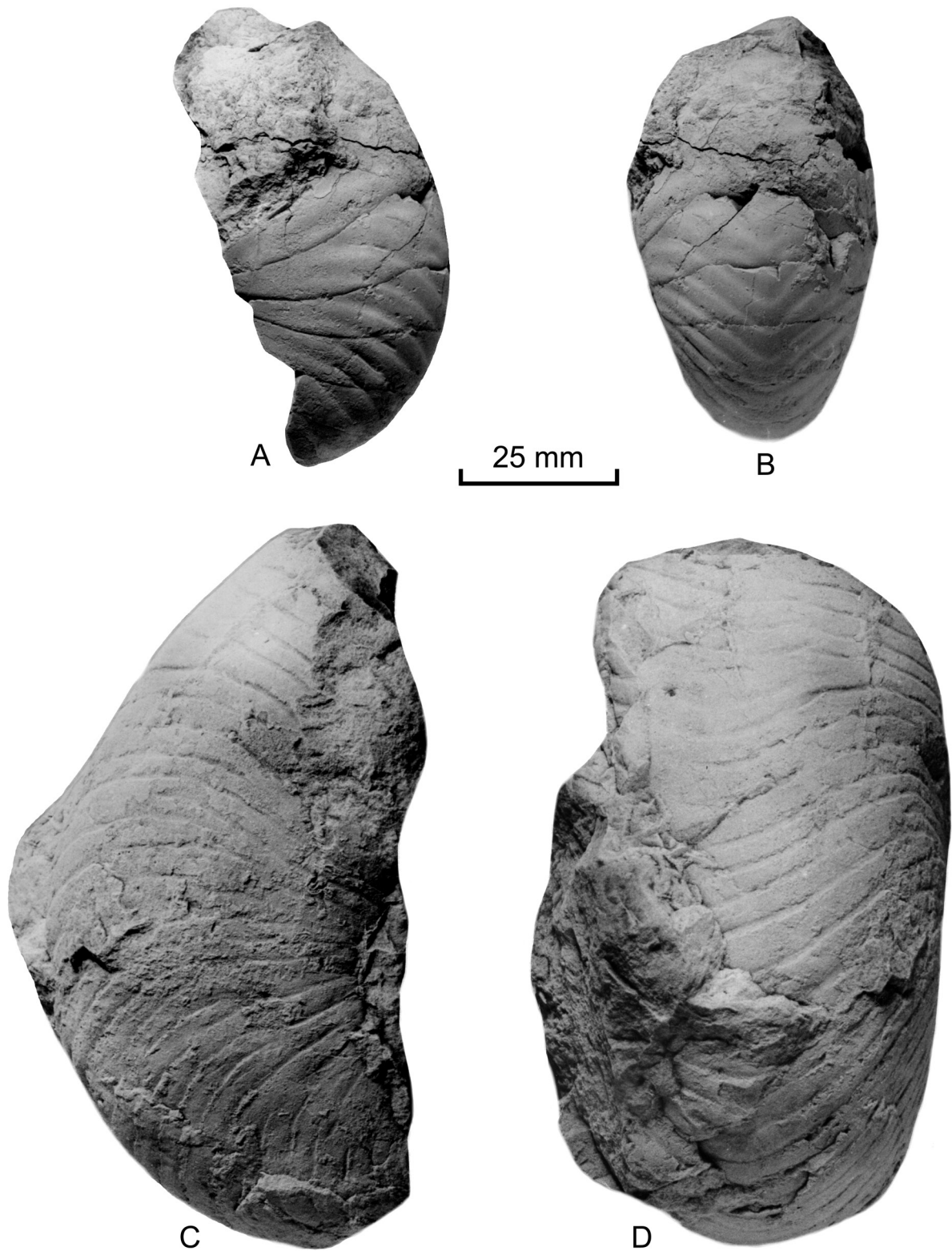
Text-Fig. 5. Cymatoceras sakalavum (COLLIGNON, 1949), A, B, GBA 2016/003/0001; C, D, GBA 2016/003/0003. Figures are x 1.
