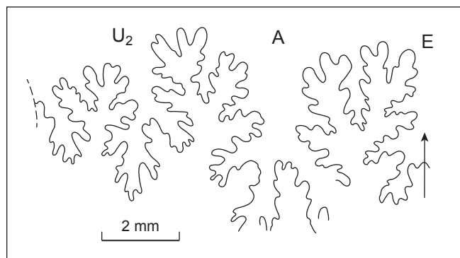
Text-Fig. 7. Partial external suture of Puzosia (Anapuzosia) sp. GBA 2016/003/0012.
