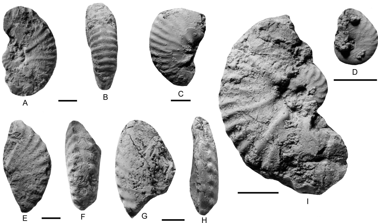
Text-Fig. 13. A–D, I: Stoliczkaia (Lamnayella) juigneti WRIGHT & KENNEDY, 1978. A, B, I: GBA 2016/003/0023; C: GBA 2016/003/0024; D: GBA 2016/003/0022, E–H: Utaturiceras sp. E, F: GBA 2016/003/0038; G, H: GBA 2016/003/0039. Figures A–C, E–H are x 1; D and I are x 2.
