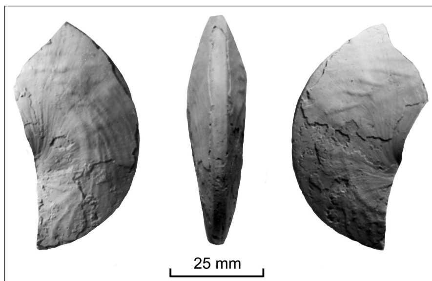
Text-Fig. 4. Forbesiceras sp. GBA 2016/004/0009, km 5.4, from the Middle or lower Upper Cenomanian part of the Odukpani Formation between Odukpani and Itu, Cross River State, Nigeria. All figures are natural size.
