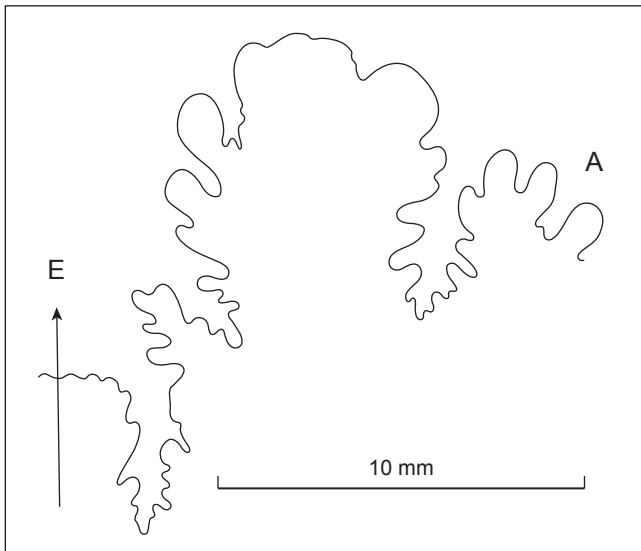
Text-Fig. 7. Cunninghamoniceras meridionale (STOLICZKA, 1864), external suture of GBA 2016/004/0036.
