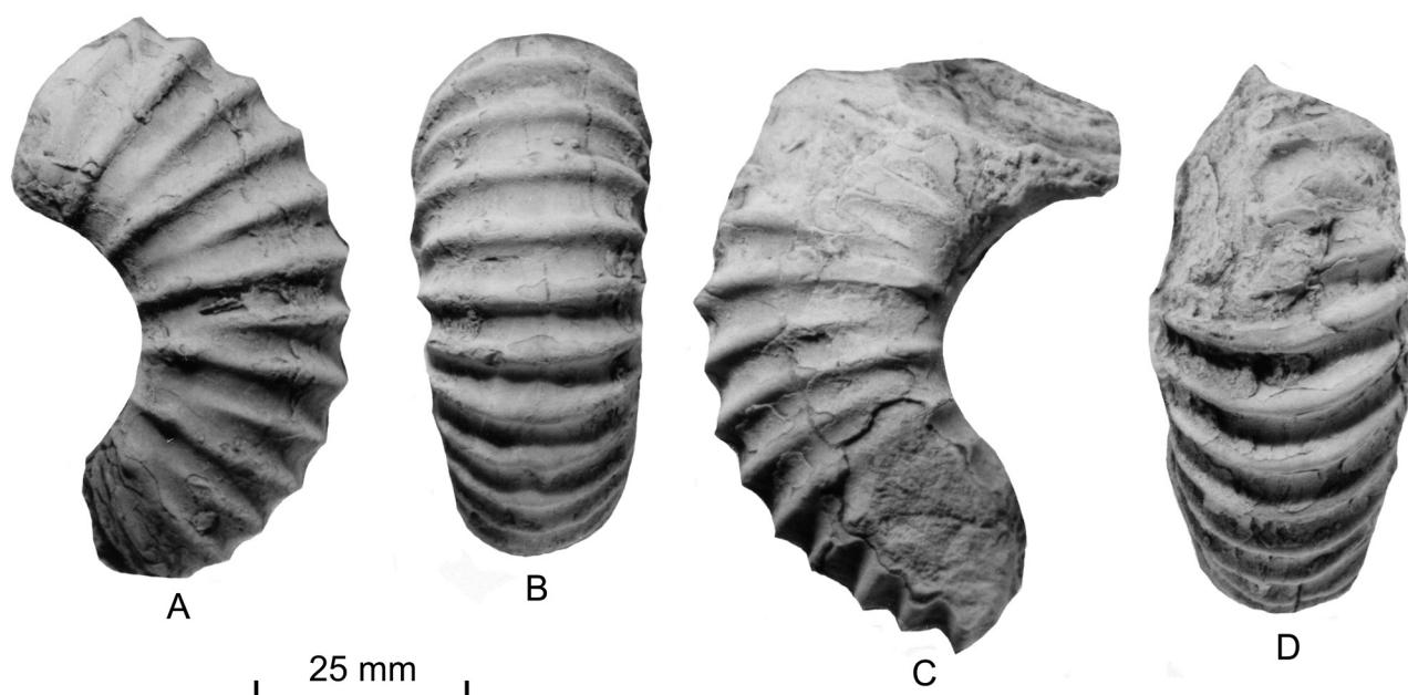
Text-Fig. 10. Calycoceras ( Gentoniceras ) sp., group of gentoni (BRONGNIART, 1822). A, B: GBA 2016/004/0042; C, D: GBA 2016/004/0043. Both specimens are from the Odukpani Formation at km 4.5, between Odukpani and Itu, Cross River State, Nigeria. All figures are natural size.
