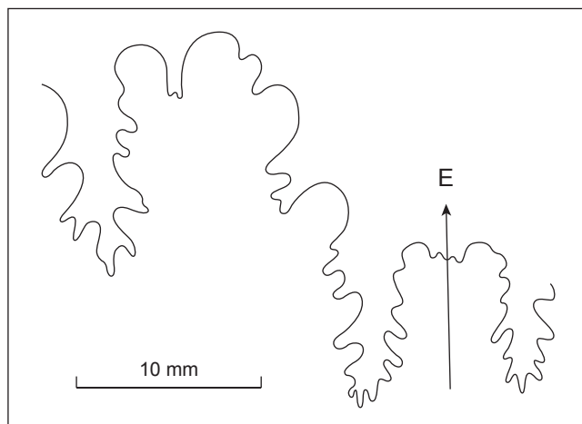
Text-Fig. 6. Cunningtoniceras meridionale (STOLICZKA, 1864), external suture of GBA 2016/004/0013.
