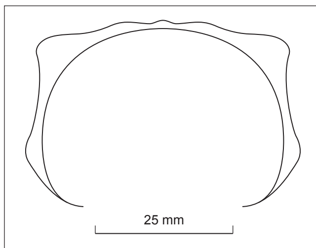
Text-Fig. 5. Cunningtoniceras meridionale (STOLICZKA, 1864), whorl section of GBA 2016/004/0013.
