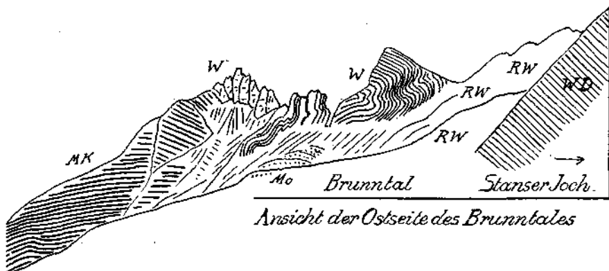
Fig. 4. RW = Rauhwacken. MK = Muschelkalk. WD = Wettersteindolomit. WK = Wettersteinkalk. Mo = Moränenwälder.
