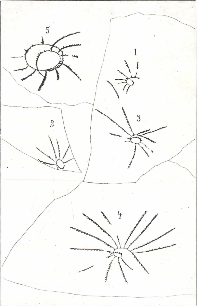
Cyrtograptus ruthenicus (nov.) Eisel.
