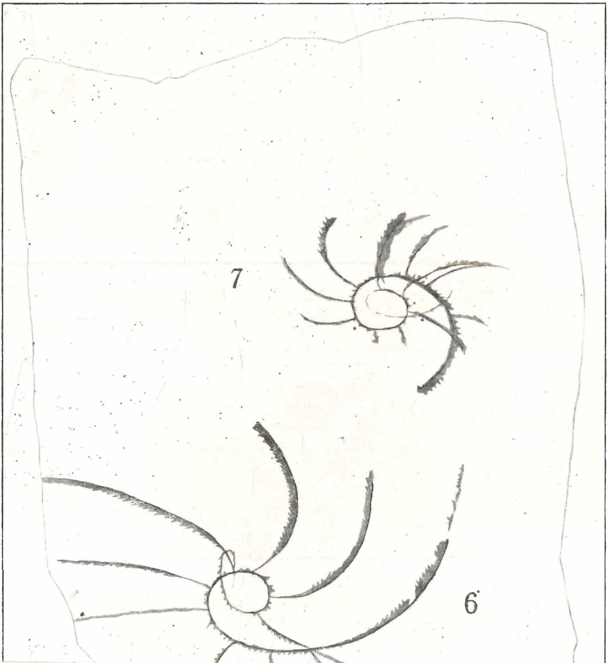
Cyrtograptus ruthenicus , var. polybus (nov.) Eisel.
