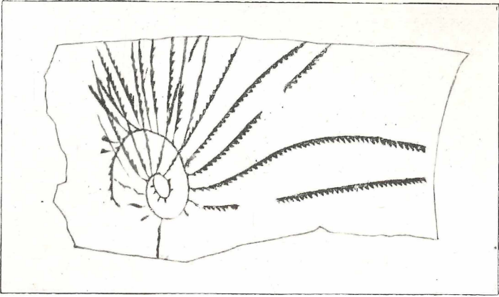
Cyrtograptus ruthenicus , var. polybus (nov.) Eisel.
