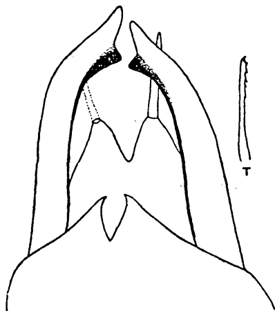
Metrioptera bodenheimeri sp. n., end of abdomen. T = titillator.
