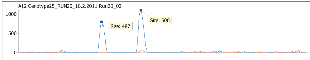
Abb. 10: Dryopteris carthusiana (DE385; Bergatreute) – Fig. 10–12: Electropherograms of PgiC 15/16 fragments of D. xdevereri and its parental species.
