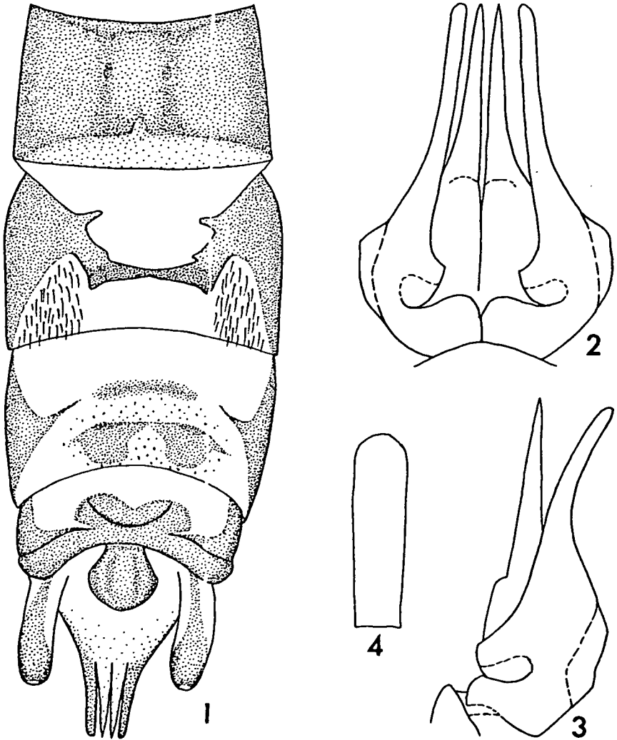
Abb.1-4: Leuctra holzschuhi sp.n. - 1. Abdomenende, dorsal; - 2. Paraprocte, caudal; - 3. Paraprocte, lateral; - 4. Bauchblase, ventral.
