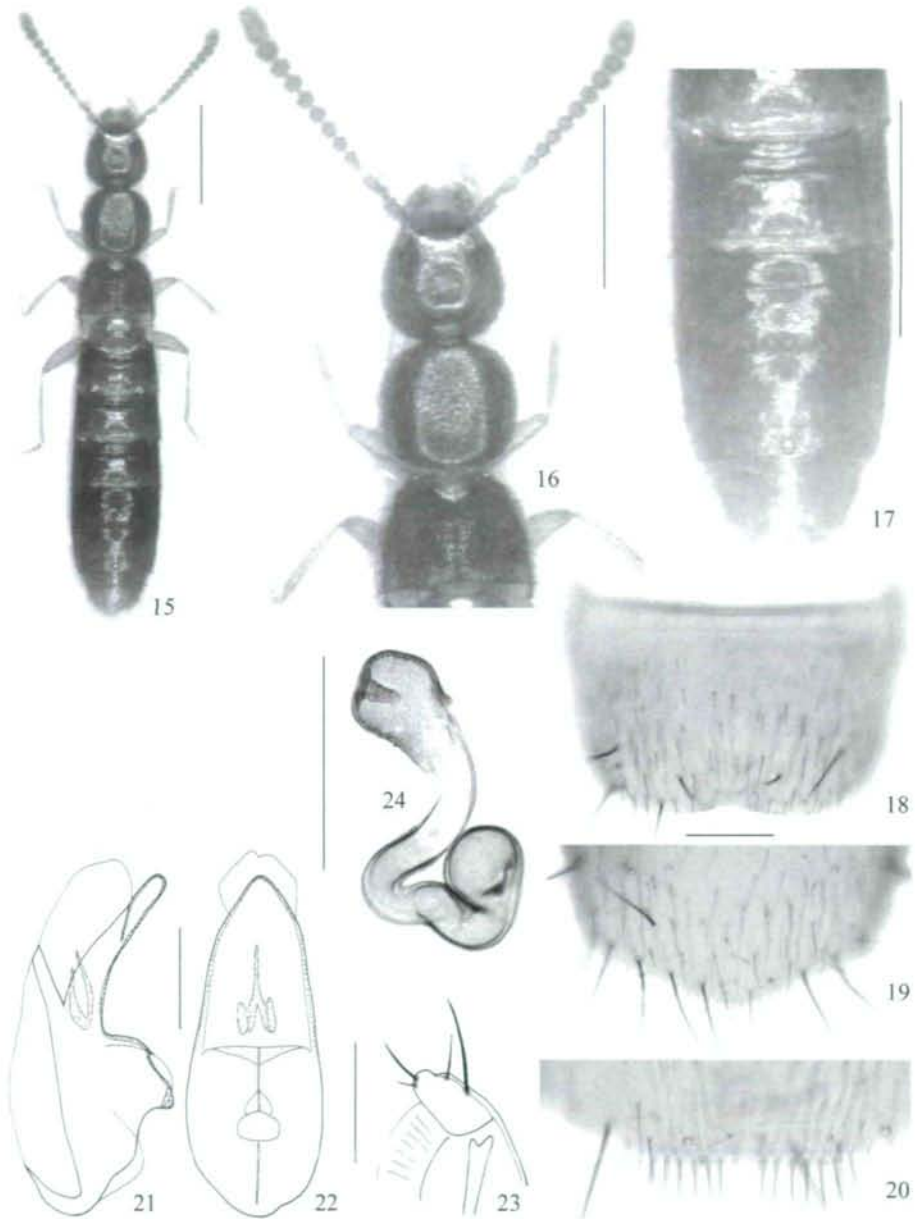
Figs. 15-24: Geostiba vidua PACE: 15 – facies ( \delta ); 16 – \delta forebody in dorsal view; 17 – posterior part of \delta abdomen in dorsal view; 18 – \delta tergite VIII; 19 – posterior part of \delta sternite VIII; 20 – posterior part of \delta sternite VIII; 21, 22 – median lobe of aedeagus in lateral and in ventral view; 23 – apical lobe of paramere; 24 – spermatheca. Scales: 15 - 17: 0.5 mm; 18 - 24: 0.1 mm.
