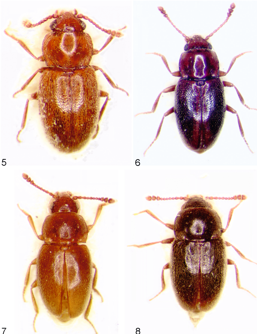
Figs 5-8: (5) Mnioticus scotti nom. nov., female; (6) Mnioticus jeanneli (SCOTT, 1936), male; (7) Mnioticus ruwenzoriensis nov.sp., pale specimen, paratype, male; (8) Mnioticus ruwenzoriensis nov.sp., dark specimen, paratype, female.
