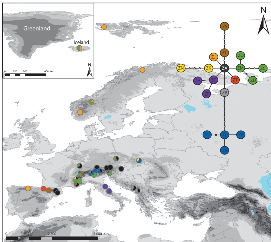
Fig. 2. – Statistical parsimony network based on trnH-psbA cpDNA sequences of Potentilla crantzii and distribution of the cpDNA haplotypes in Europe. Small empty circles represent haplotypes that are not present, but necessary to link all the haplotypes recorded to the network. All haplotypes are separated from the nearest haplotype by one mutation/indel.
