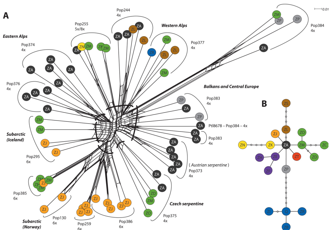
Fig. 3. – Phylogenetic relationships among individuals of Potentilla crantzii based on AFLP and cpDNA data. A. Neighbor-Net dendrogram based on Jaccard distances among AFLP genotypes with chloroplast haplotypes depicted on corresponding branch tips. The scale bar indicates genetic distance. Bold lines indicate geographic groups written in bold italics. B. Statistical parsimony network based on trnH-psbA cpDNA sequences.
