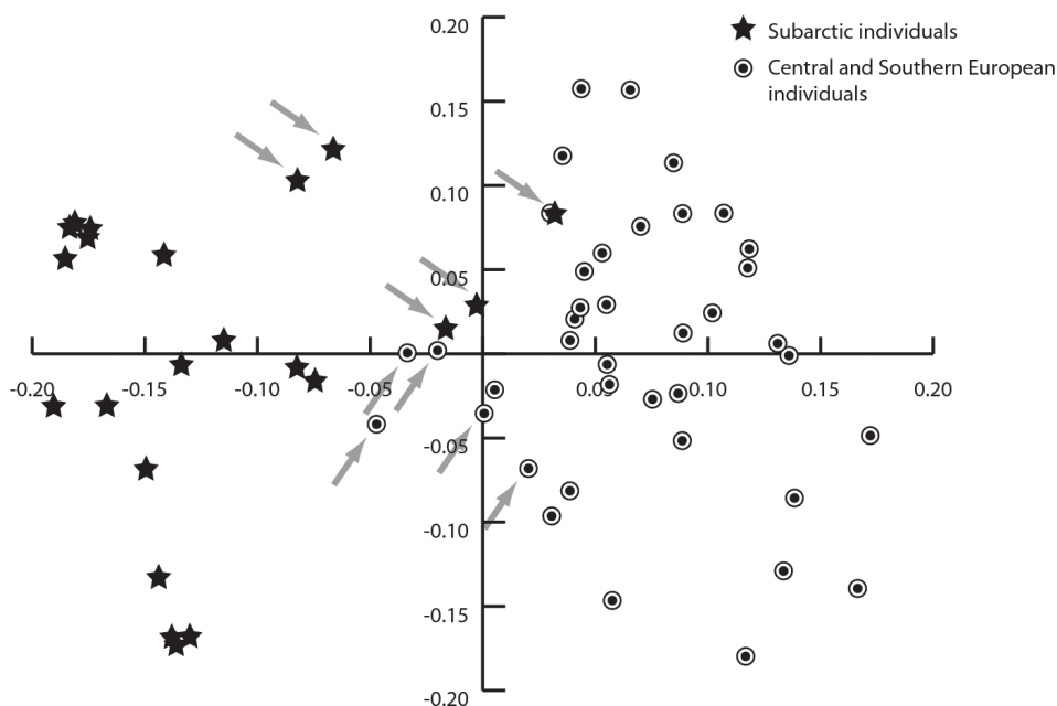
Fig. 5. – Principal co-ordinate analysis (PCoA) of AFLP genotypes of Potentilla crantzii . The first two axes explained 15.23% and 9.39% of the total variation, respectively. Arrows denote the lowland serpentine population in the Czech Republic (Pop375) and subarctic population in Iceland (Pop295). The genetically highly distinct tetraploid Pop384 (Montenegro) was excluded from this analysis.
