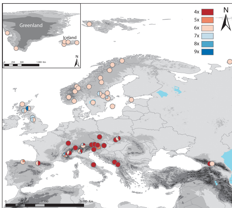
Fig. 1. – Map showing the distribution of cytotypes of Potentilla crantzii in Europe based on both newly acquired and previously published data (see Electronic Appendix 1 for a complete list). Pie charts are proportional to the frequency of a particular cyotype recorded in one population or in several closely adjacent populations (up to 65 km).
