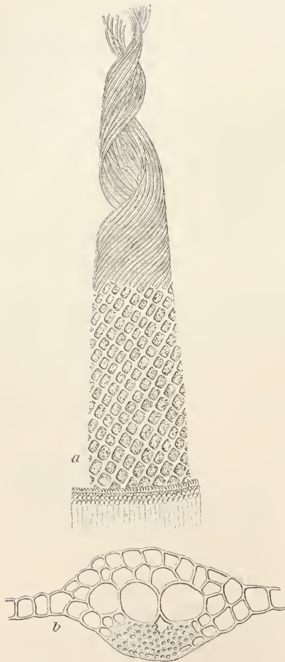
Tortula subulata . a Basale Blatt- rippe, b Peristom \frac{1.0.0.}{4} .
