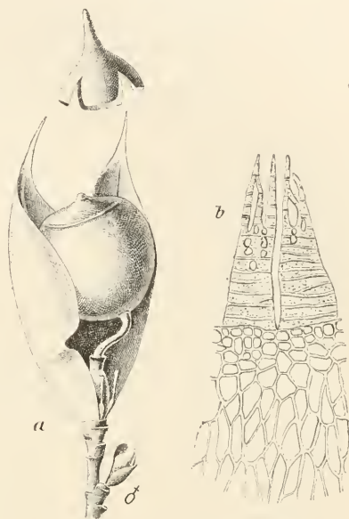
Grimmia plagiopodia Hedw.
