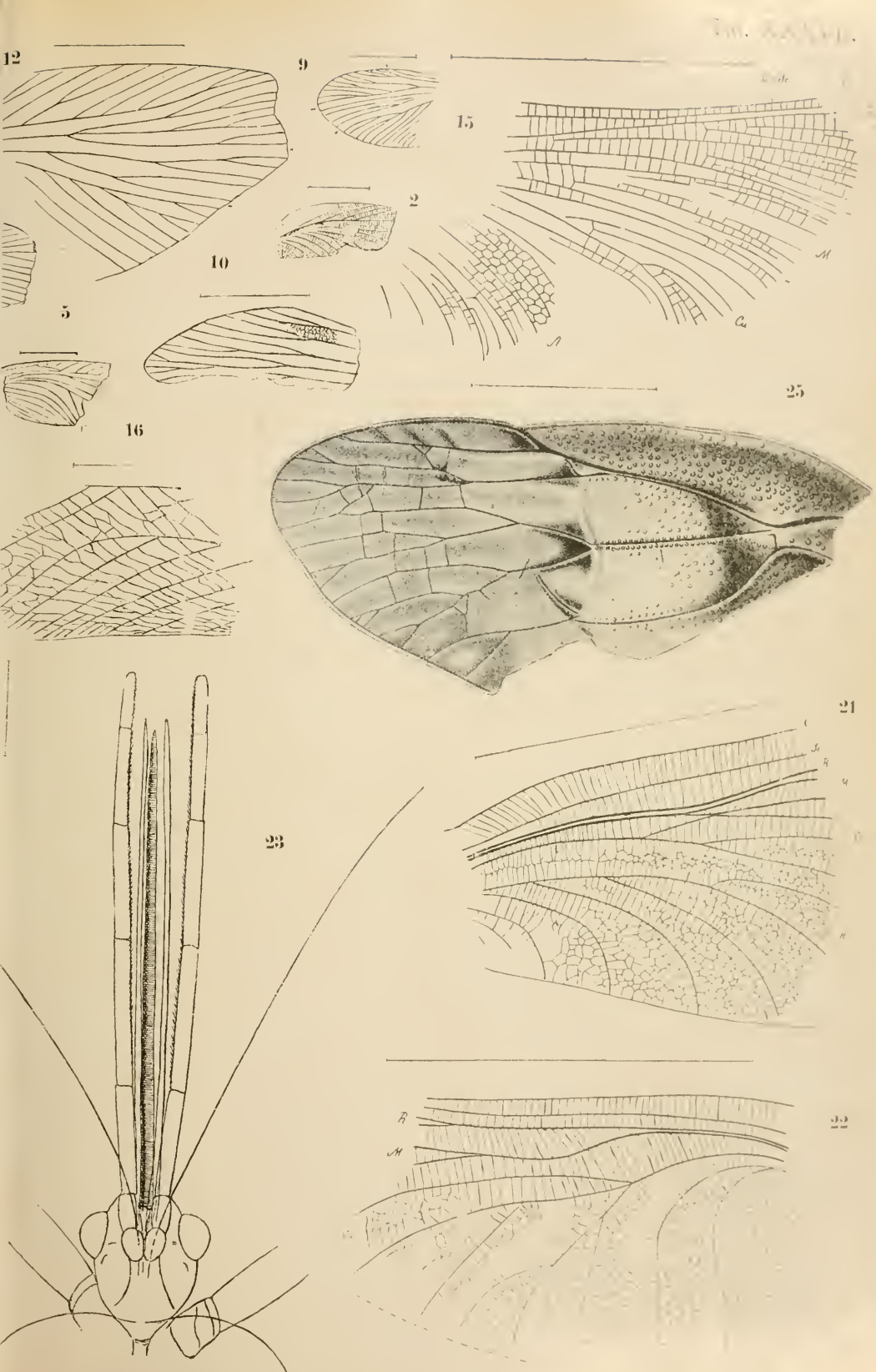
1) - Protohemiptera (21-23) - Palaeohemiptera (24-27) in C. L. ...
