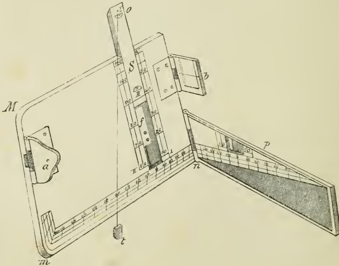
Fig. 443. Faustmann's Spiegelhypsometer.
