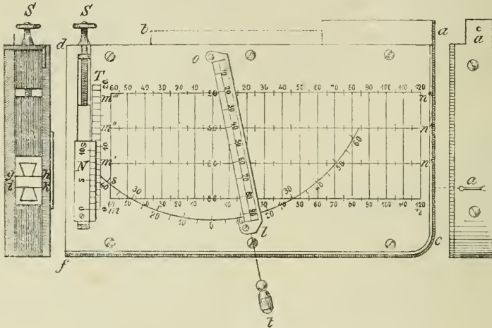
Fig. 442. Winkel's Dendrometer.
