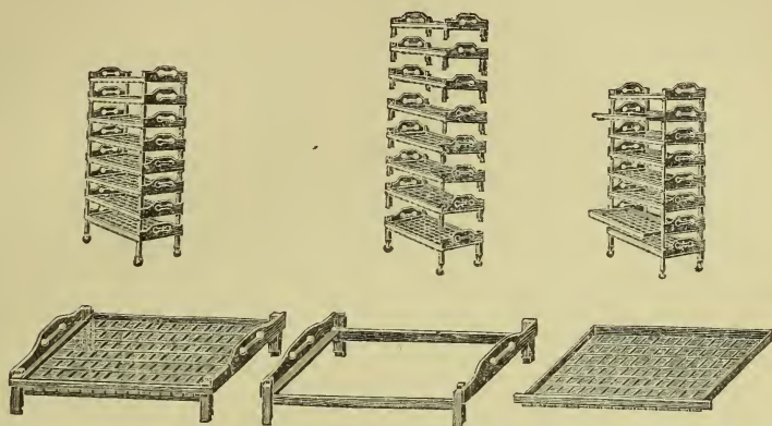
Fig. 275. Obst-Universal-Gestell.
