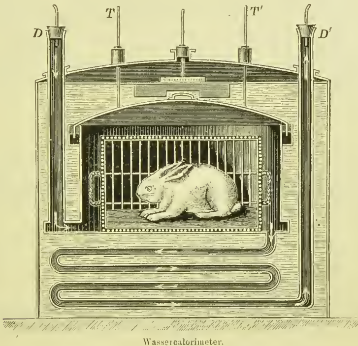
Wassercalorimeter.
