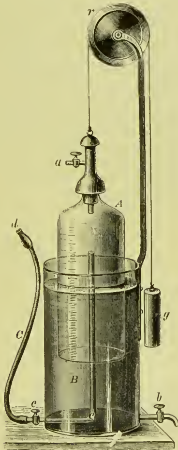
Spirometer.
