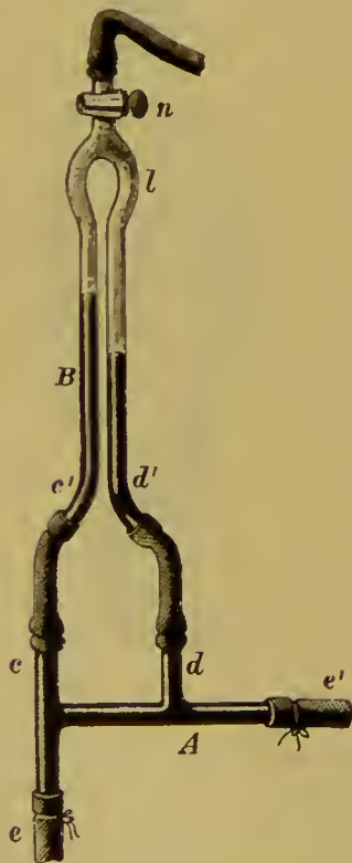
Cybulski's Photohaemotachometer.
