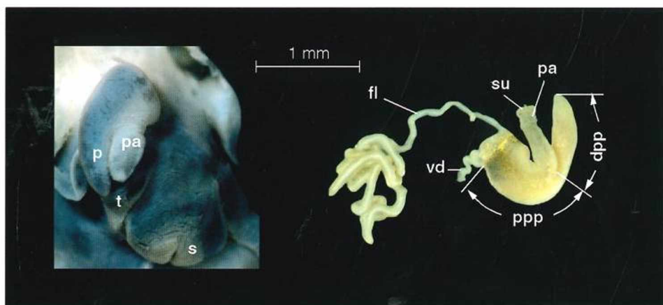
Fig. 2. The Morphology of the penis of Bithynia species ( B. mostarensis Moellendorf, 1873). fl=flagellum, dpp=distal part of the penis, p=penis, pa=penial appendix, ppp=proximal part of the penis, s=snout, su=sucker, t=tentacle, vd=vas deferens (after GLOER & PEŠIĆ, in press).
