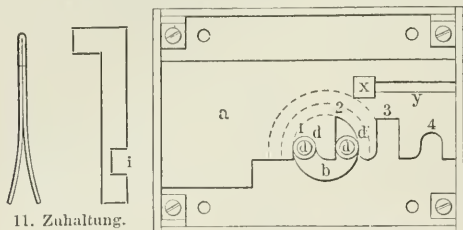
8. Bramah-Schloß.
