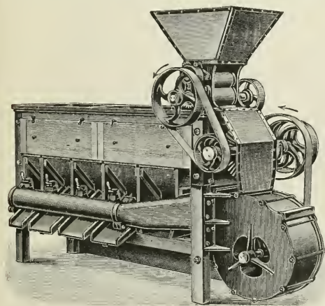
2. Brechmaschine.
