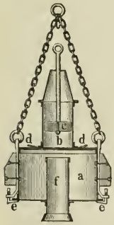
Sandpumpe.
