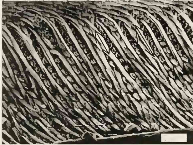
Fig. 17: Uniserial arrangement of the enamel as observed in a longitudinal section of the incisor enamel of Mus musculus (House Rat), showing distribution of the HSBs and the outer enamel. Arrow marks the direction of the maximum tensile stresses observed in the rodent incisor enamel under the gnawing load condition. Scale bar = 10 microns. Anterior part (incisal direction) of the incisor is towards the left side of the photograph.
