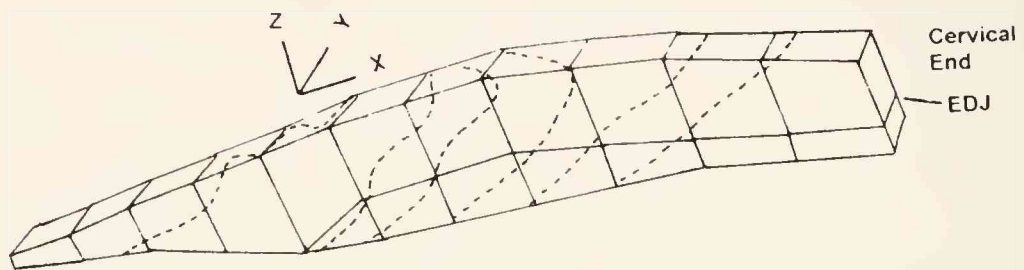
Fig. 11: Curved chisel shaped incisor showing direction of the cracks as inferred from the direction of maximum tensile stresses produced due to the gnawing load.
