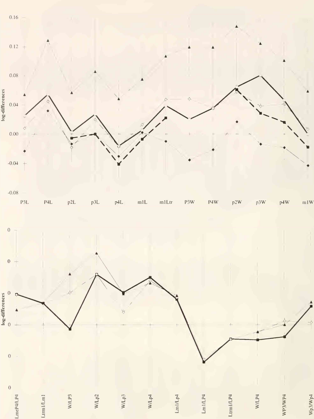
Fig. 9: Logarithmic ratio-diagram, comparing the teeth dimensions (a) and teeth indices (b) of Pliocrocota perrieri arambourgi from Sarikol Tepe, Turkey with several Plio-Pleistocene “crocutoid” hyaenas. Standard= P. pyrenaica , Perpignan, France (orig. meas.) ■ Pliocrocota perrieri arambourgi from Sarikol Tepe, Turkey ; 8b: mean values ◆ Pliocrocota from Odessa Catacombs, Ukraine ◇ P. perrieri mean (data from HOWELL & PETTER 1980) ▲ P. brevirostris from Europe mean “
