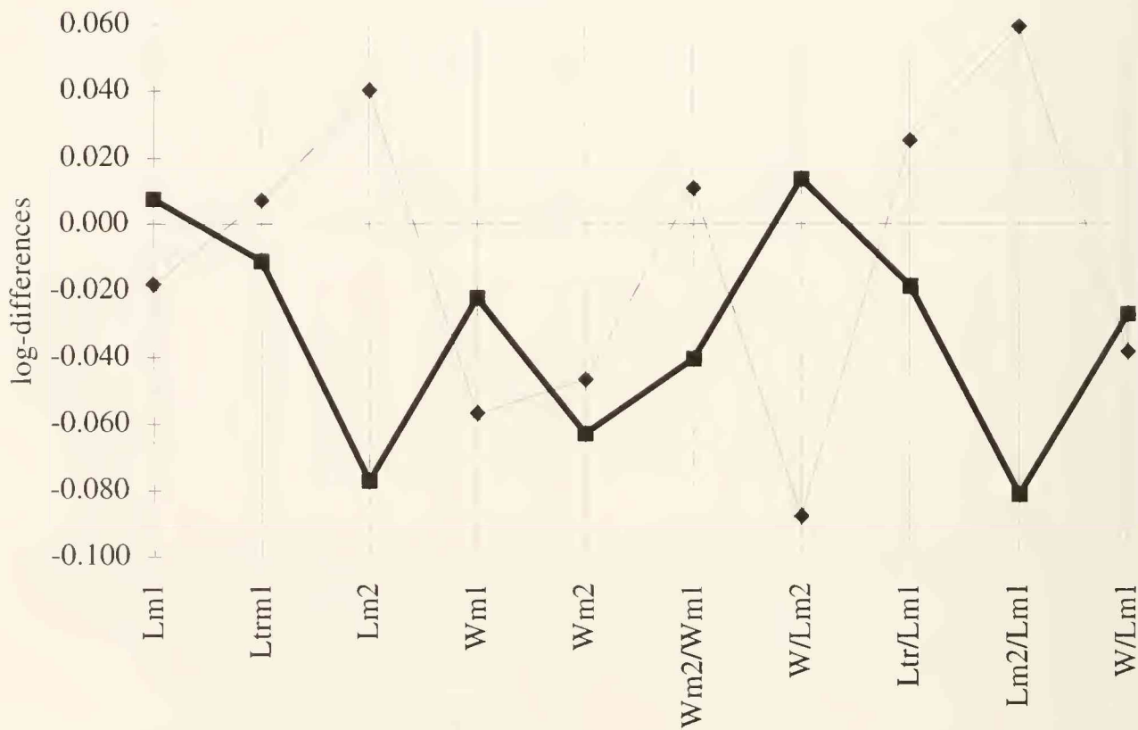
Fig. 6: Logarithmic ratio-diagram, comparing the lower teeth dimensions of Eucyon cf. odessanus (■) from Sarikol Tepe with Eucyon davisi (◆) from Alatini, Greece (data from ROOK 1993; KOUFOS 1998). Standard= Eucyon davisi (mean) from Bird Bone, N. America.
