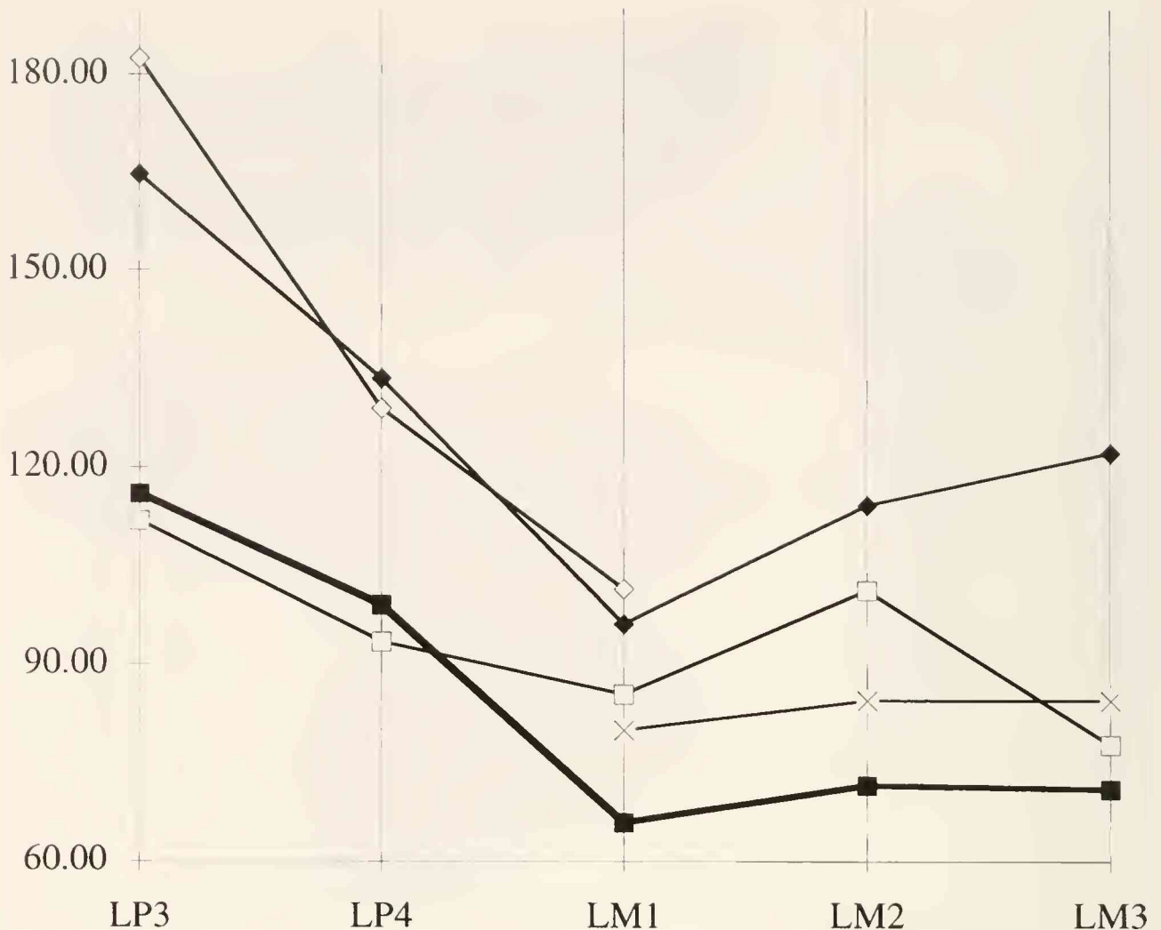
Fig. 20: Percentage ratio diagram comparing the teeth dimensions of several Plio-Pleistocene camelids. Standard= Camelus bactrianus (data from LESBRE 1900). ■ Paracamelus cf. alutensis from Sarikol Tepe, Turkey ◆ P. gigas (data from ZDANSKY 1926) ◇ P. gigas from Nihowan, China (data from TEILHARD & TRASSAERT 1937) □ P. alexjevi (data from KHAVESON 1954) × Camelus dromedarius (data from LESBRE 1900)
