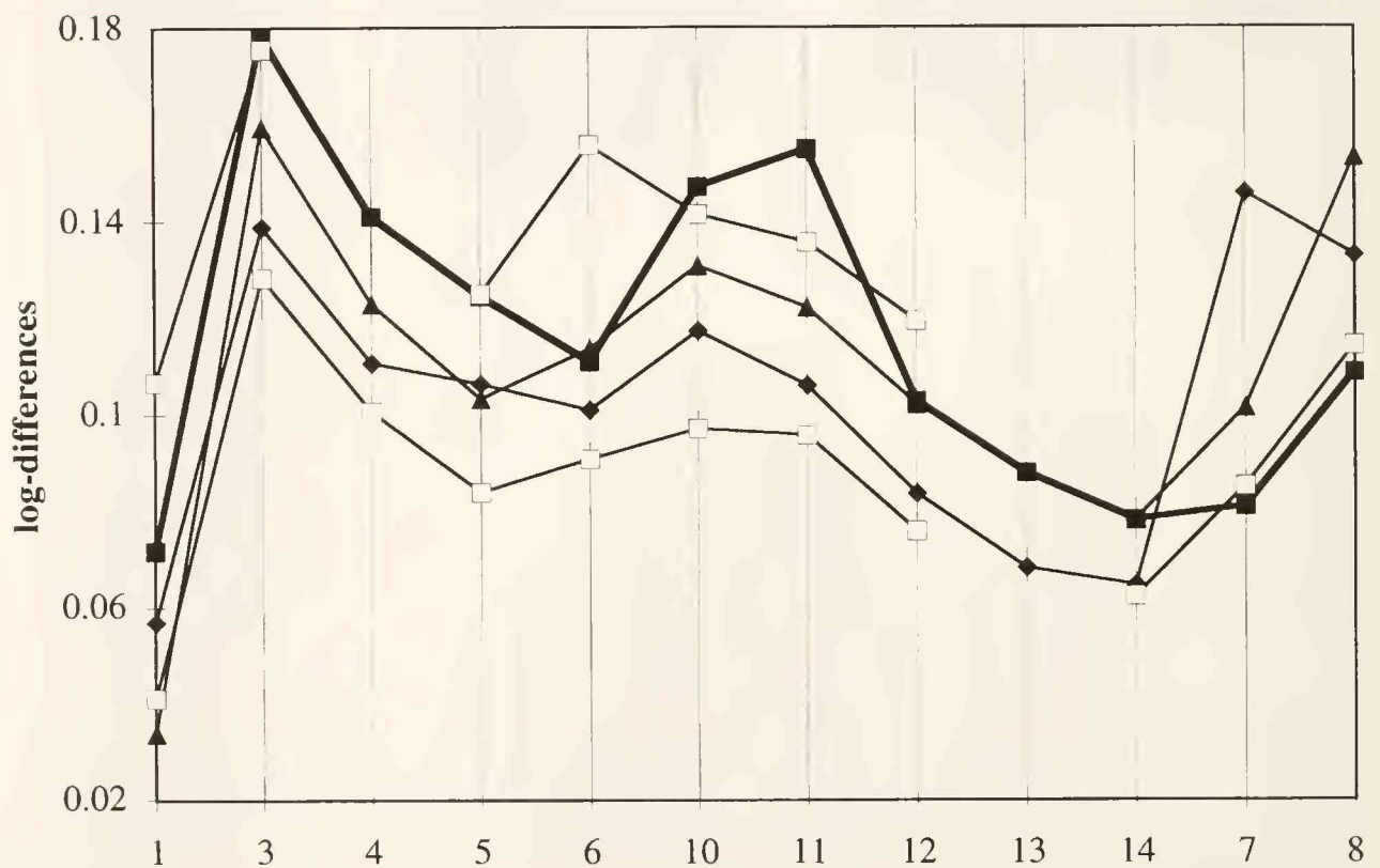
Fig. 15: Logarithmic ratio-diagram, comparing the metacarpal dimensions of Equus stenonis from Sarikol Tepe, Turkey, with several Plio-Pleistocene equids. Standard= E. hemionus onager , mean values, EISENMANN 1979.
