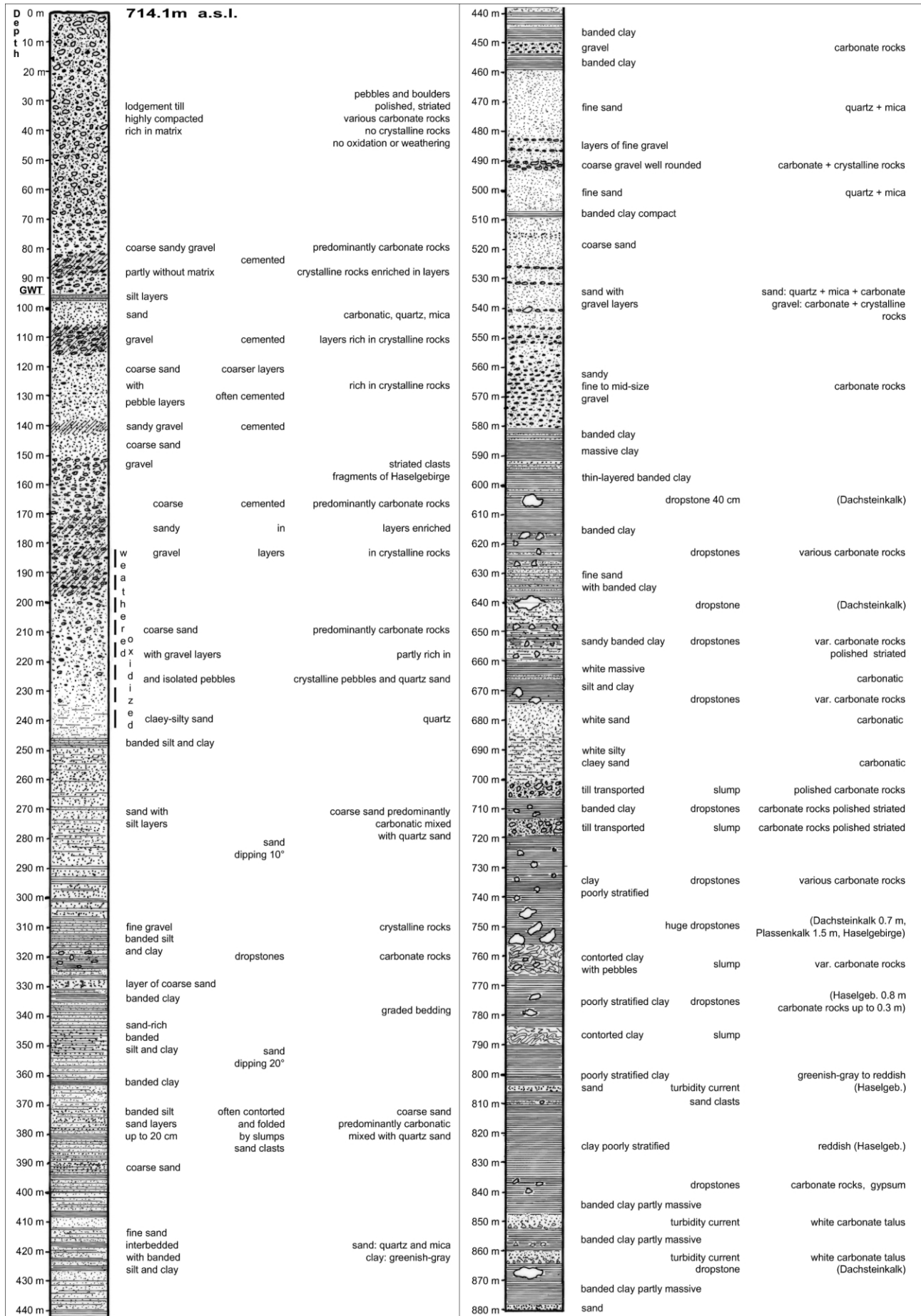
FIGURE 3: Condensed description of the sediment sequence of the exploratory drilling (Reitern 1).
