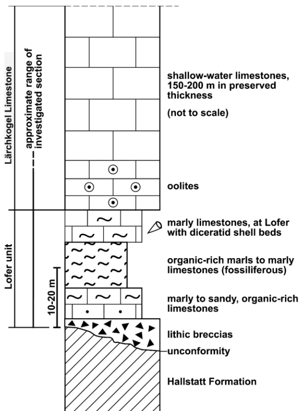
FIGURE 2: Schematic generalized section of Lofer unit and its lateral correlatives in the environs of Lofer, and overlying Lärchkogel limestone, respectively (modified from Ferneck, 1962, and Lukesch, 2003).
