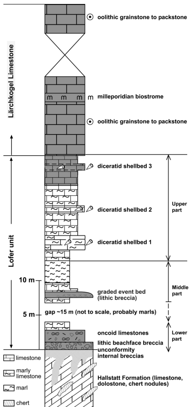
FIGURE 3: Section of Lofer unit immediately north of village Lofer. The approximate position of the 'graded event bed (breccia)' as described in the text has been laterally projected over a distance of about 15 m into the section. Higher above, diceratid rudists are abundant in three distinct shell beds. The subdivision of the Lofer unit into a lower, middle and upper part, respectively, refers to the description of the section in the text.
