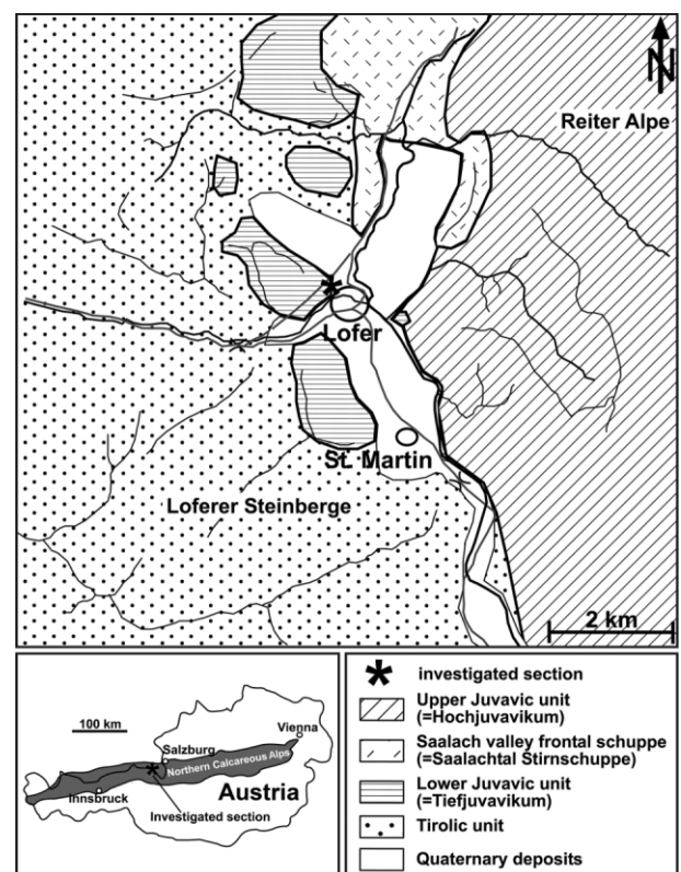
FIGURE 1: Position of investigated succession in Austria (inset), and geological map of environs of Lofer (simplified from Lukesch, 2003).
