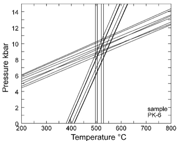
FIGURE 7: P-T estimates of sample PK-6 based on the Fe – Mg exchange reactions between garnet 2 and phengite and garnet 2 and biotite and the net transfer reaction garnet 2 – muscovite – plagioclase 2 – quartz.
