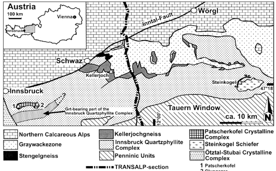
FIGURE 1: Geological overview of the area of investigation. Note the TRANSALP section in the center of the image crosscutting all tectonic units.
