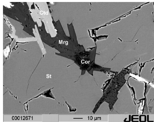
FIGURE 2: This BSE image shows the breakdown of staurolite (St) to chloritoid (Ctd) + margarite (Mrg) according to reaction (1) (sample PK-5). Within chloritoid, corundum (Cor) occurs.
