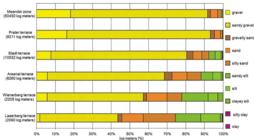
FIGURE 5: Cumulative thickness of gravel, sand, silt and clay layers within Quaternary units (modified after Pfliederer and Hofmann, 2007).
