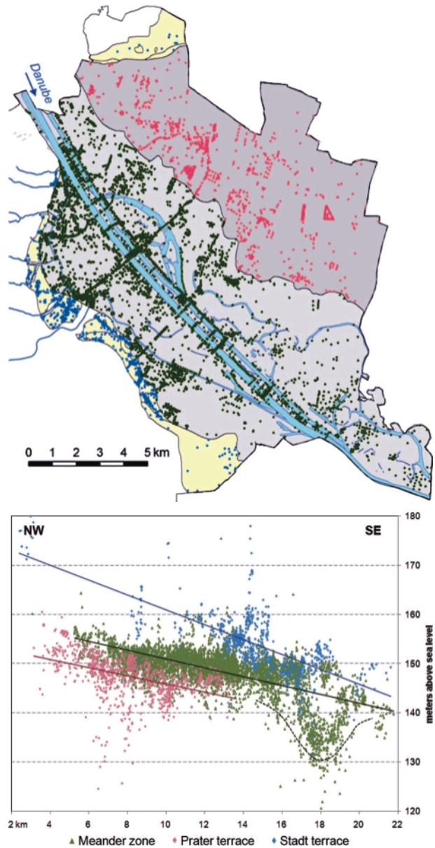
FIGURE 3: Trends of base elevation for the three youngest gravel units along the direction of ancient river flow (bottom). Location of boreholes used for analysis (top). Downward gradients amount to 1.5 ‰ for the Stadt terrace and 0.8-0.9 ‰ for the Prater terrace and the Meander zone. Dotted line indicates area of tectonic subsidence (Schwechat). (modified after Pfeleiderer, 2008).
