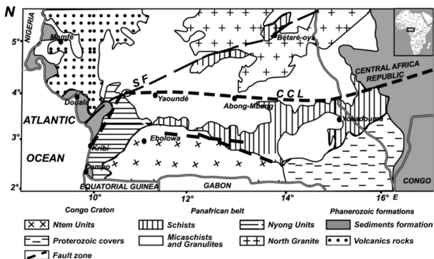
FIGURE 1: Geological sketch map of the southern Cameroon region. The major structural units shown are the Congo craton, the Pan-African belt, some Cretaceous to recent sediment (Mamfe, Douala-Kribi-Campo and Central Africa Republic) and volcanic rocks; SF: the Sanaga Fault; CCL: the northern Congo Craton Limit.
