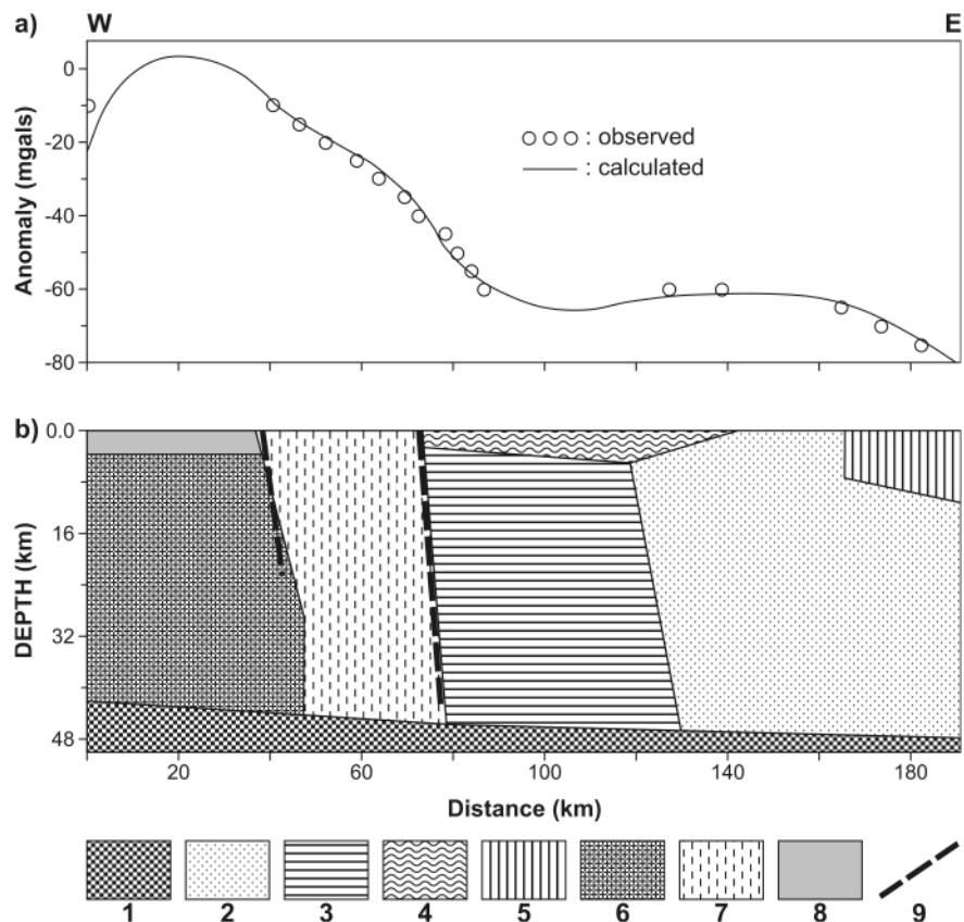
FIGURE 6: Bouguer gravity model of E-W profile of Fig. 3. The upper panel shows calculated and observed Bouguer gravity, and lower section shows the preferred model distributions.
