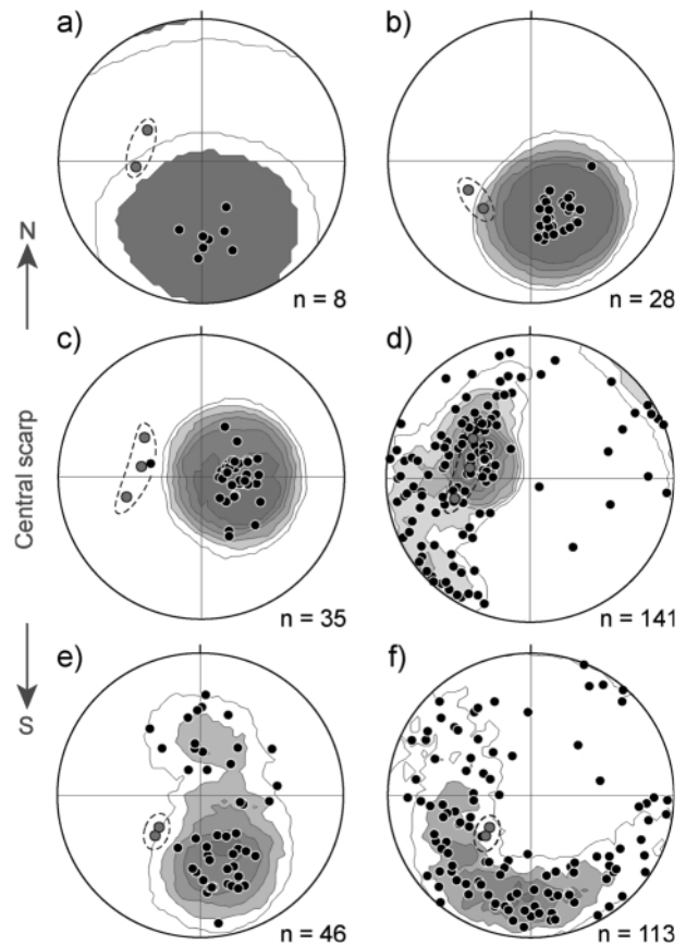
FIGURE 5: Measured discontinuities (black, poles to planes, lower-hemisphere) and mean slope orientation (grey, poles to planes, stippled enveloped) of the Köfels rockslide scarp area: foliation of a) paragneisses in the northern scarp area (Wenderkogel), b) para- and orthogneisses at the slope northeast of Köfels, c) orthogneisses in the central scarp area and e) paragneisses in the southern scarp area (Hohe Seite), as well as fractures of d) orthogneisses in the central scarp area and f) paragneisses in the southern scarp area.
