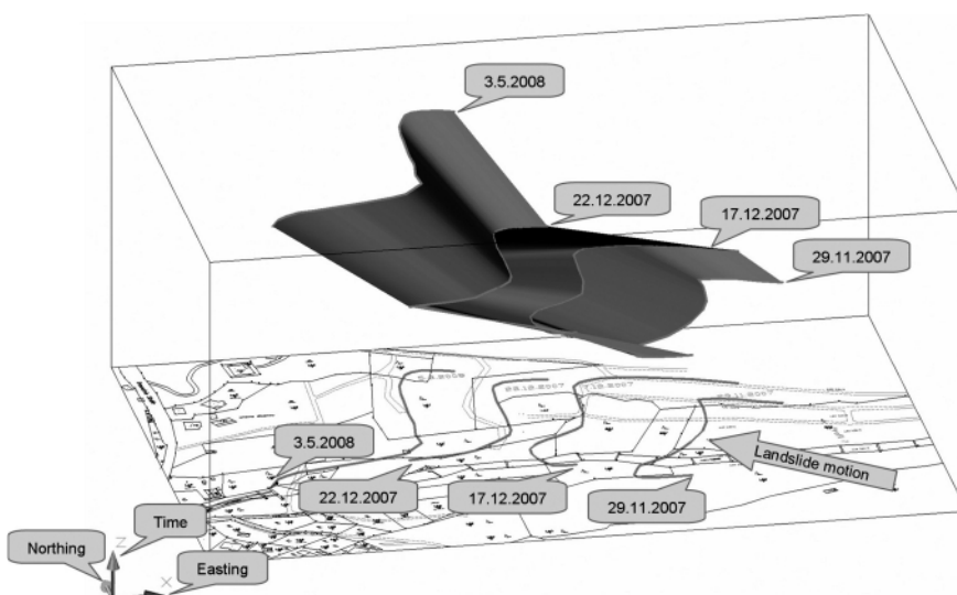
FIGURE 9: Development of a discontinuity zone on a map (bottom) and in the space-time prism (top). Bottom: traces of evolving shear zone, as mapped by the geologist on the Gschliefgraben landslide surface on different dates. Superimposed space-time prism: abstraction of the evolving shear zone as a surface, which acts as a boundary condition for space-time Kriging. See text for details.
