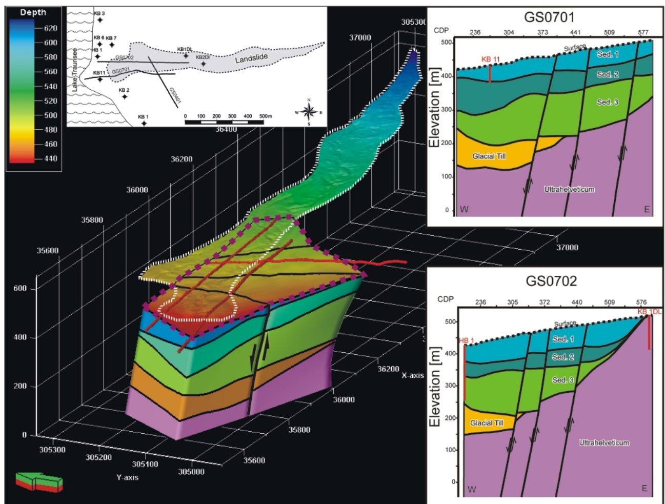
FIGURE 5: Final model derived from seismic reflection data. The red lines indicate the seismic profiles according to the basemap. The black lines at the surface of the model give the position of the modeled faults. The area with the dashed white border represents the most recent landslide in November 2007, while the pinkish dotted line shows the model boundary. On the right, two cross-sections along the seismic profiles GS0701 and GS0702 are shown.
