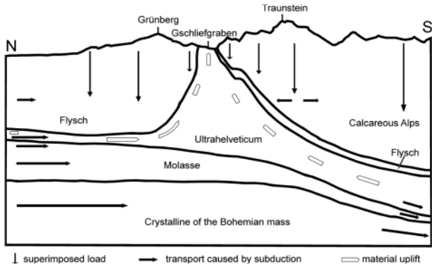
FIGURE 2: Geological north-south cross-section for the Gschliefgraben and its surroundings, modified after Daurer and Schäffer (1983).
