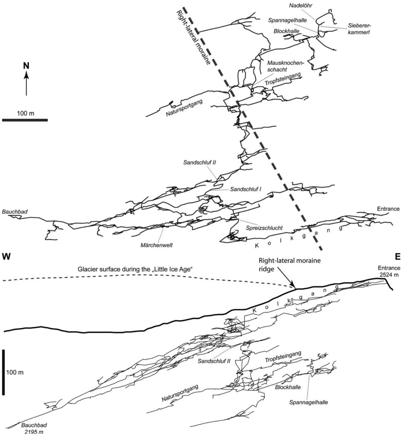
FIGURE 2: Upper panel: Plan view of Spannagel Cave and names of cave parts mentioned in the text. Note that the western segment of this cave was in a subglacial position during the "Little Ice Age" advances of the Hintertux Glacier, which currently (2010) terminates ca. 500 m south of the cave. Lower panel: Vertical perspective of the cave's dendritic network and the reconstructed surface of the glacier during its highstand in the middle of the 19 th century. The near-linear, first-order arrangement of the cave passages follows the dip the marble. Both maps show the traverses only (excluding gallery boundaries).
