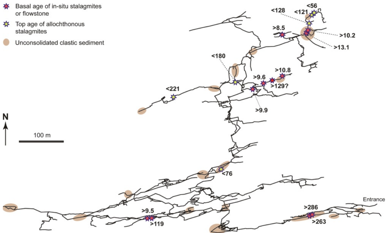
FIGURE 3: Location of the U-Th-dated speleothems discussed in this study. Ages are given in kyr. See text for further information.
