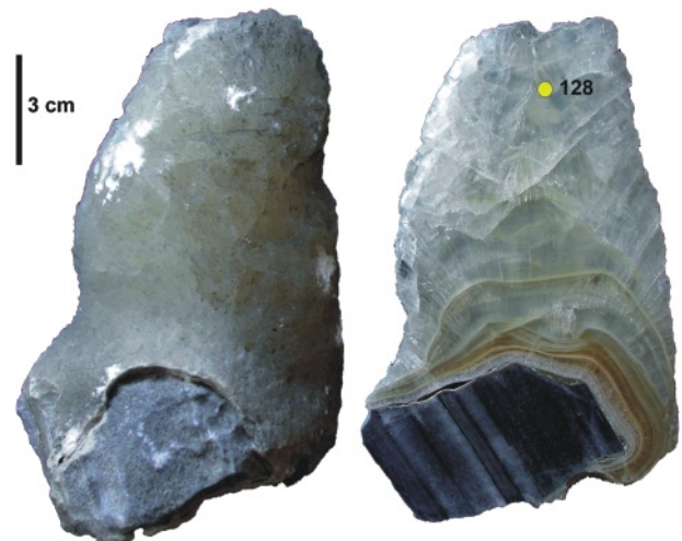
FIGURE 9: Stalagmite SPA 139 (outside left, polished slab right), found less than 30 m from SPA 51 (Fig. 10), was broken and exposed to aggressive water resulting in a dissolution-sculptured surface.
