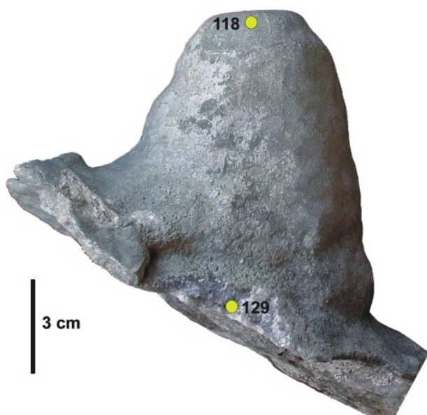
FIGURE 7: Stalagmite sample SPA 129, found in-situ in the Tropfsteingang, grew during the Last Interglacial (ages in kyr). The thin layer of gray clay on the left flank suggests either a short flooding event during the last glacial or deposition of dust.
