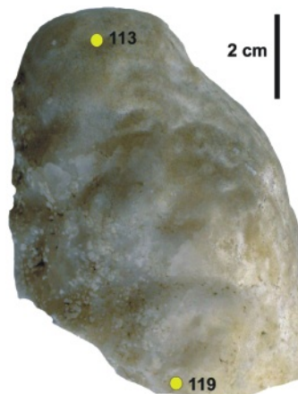
FIGURE 11: This inactive stalagmite (SPA 143) was found in growth position on a breakdown block at Märchenwelt in the western branch of Spannagel Cave. The brown loam stems from cavers who touched the specimen. The right picture shows the stalagmite after cleaning. Note smooth, uncorroded surface, demonstrating that this gallery was never flooded since the Last Interglacial (dates in kyr).
