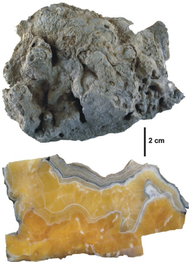
FIGURE 15: Outside (top) and inside (bottom) of a heavily corroded flowstone fragment (sample SPA 15) from the show cave part of Spannagel Cave which yielded the oldest radiometric age so far, based on U-Pb isotope data (see text).
