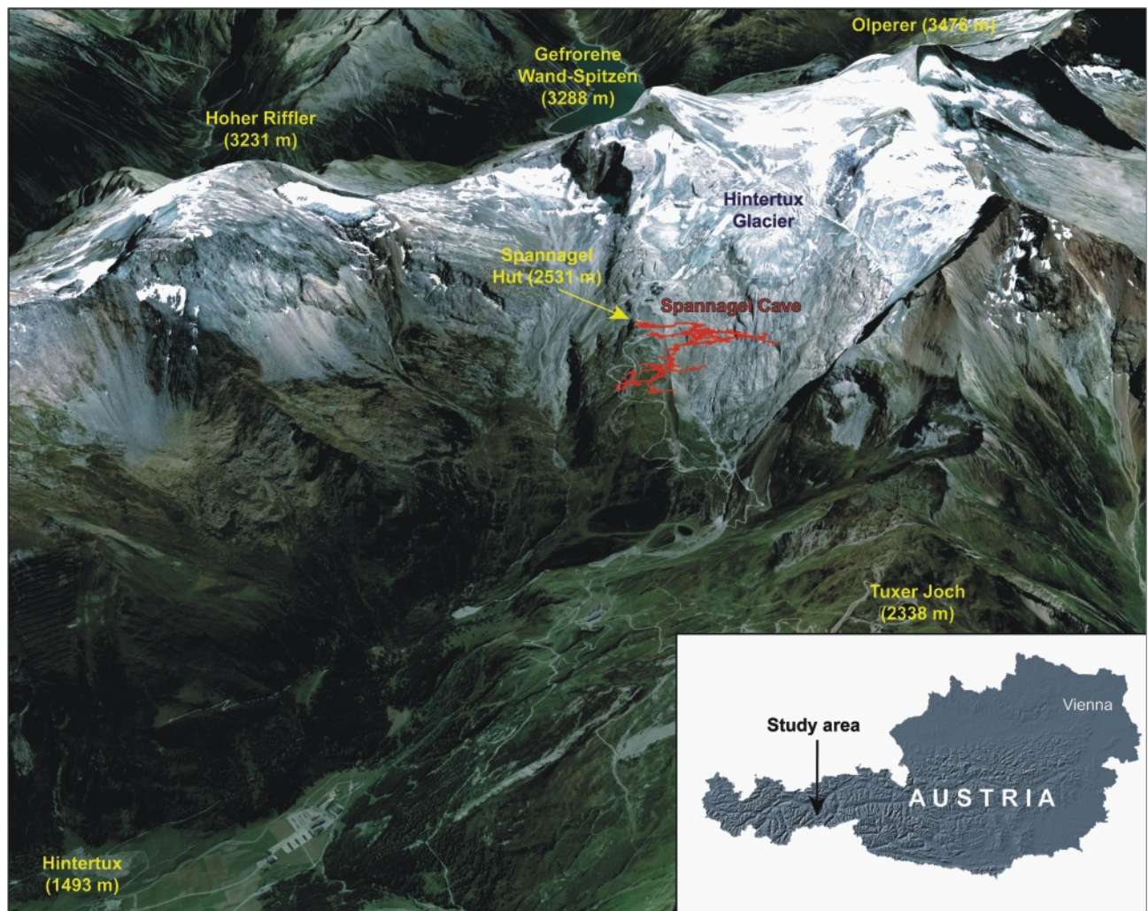
FIGURE 1: Head of the Tux Valley showing the location of Spannagel Cave adjacent to the glaciated main ridge of the Central Alps (oblique view toward SSE, satellite image downloaded from Google Earth Pro on 22 February 2010; image credit: Google Earth™ mapping service).
