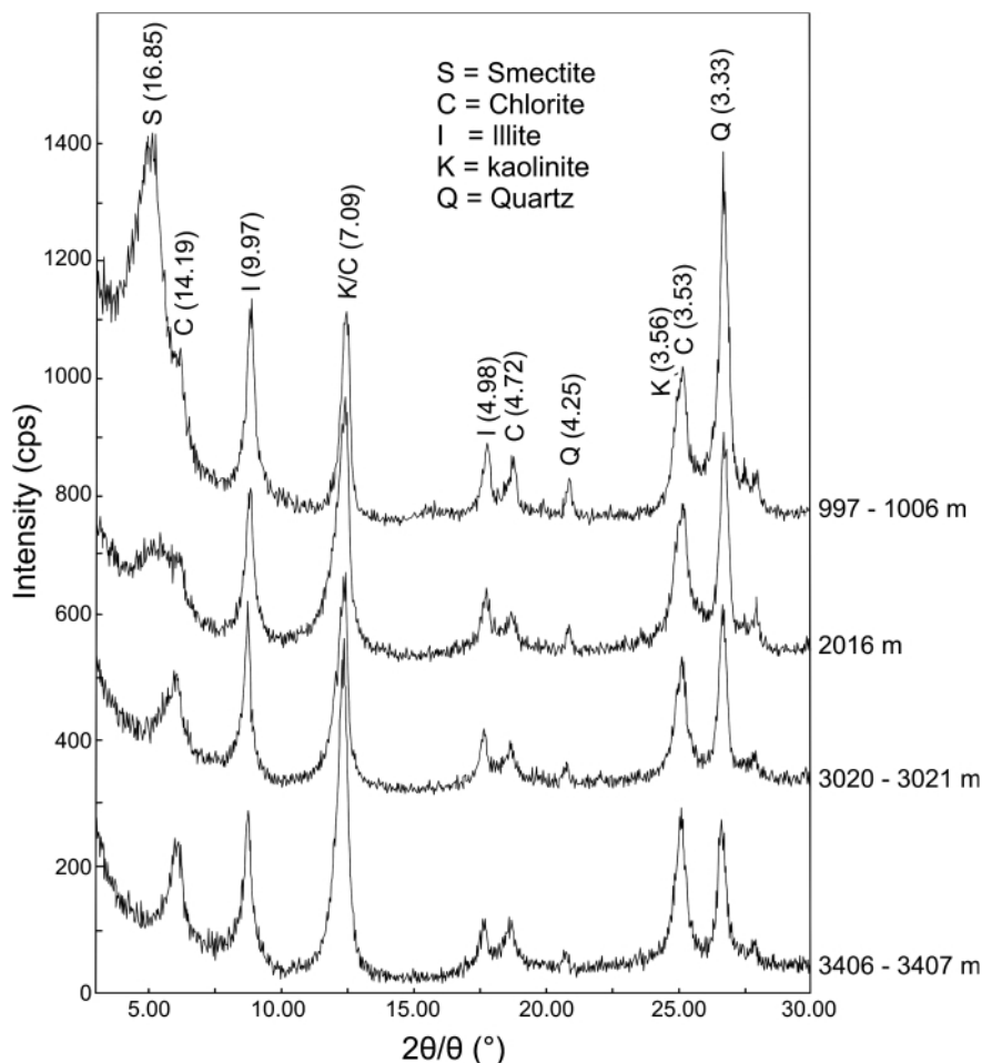
FIGURE 11: Characteristic X-ray diffraction diagrams (glycolated) of clay minerals from shale lamina within sandstones of the Surma Group from the Shahbazpur well-1.
