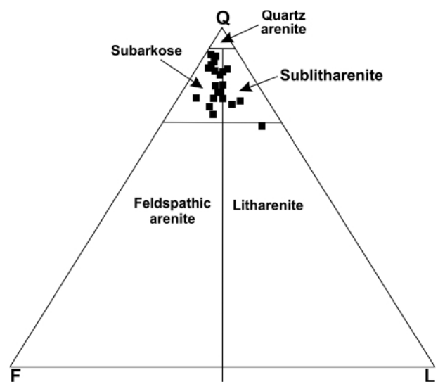
FIGURE 4: Triangular diagram (Folk, 1974) showing the modal composition and classification of the Surma Group sandstones in the Shahbazpur well-1.
