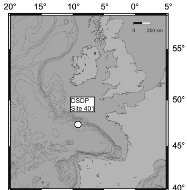
FIGURE 1: Location of DSDP Site 401 in the present-day north-eastern Atlantic (Bay of Biscay).
