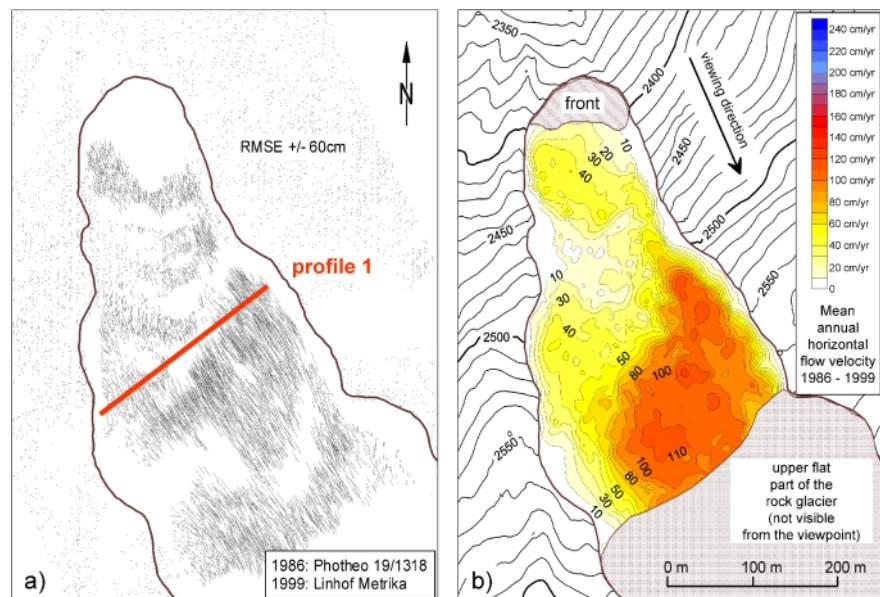
FIGURE 14: a) Horizontal displacement vectors at Äußeres Hochebenkar rock glacier derived from terrestrial photographs 1986 (Zeiss Phototheo 19/1318) and 1999 (Linhof Metrika 45). A root mean square error of \pm 60 cm in horizontal vector length was achieved, resulting in an accuracy of \pm 4.6 cm/yr. Results obtained in profile 1 (which is actually profile 1A of Figure 4b) are in good accordance with the geodetic measurements (Schneider and Schneider, 2001). Areas with low texture, dark shadows, and also excessive surface change, as well as areas which are occluded in the original photographs do not show any displacement vectors. b) Mean annual horizontal flow velocity derived from the results presented in a). A relatively inactive zone can be identified on the orographic left side of the rock glacier. The result obtained for the time period 1999-2003 (not shown in this paper) reveals a more than 200% increase in flow velocities.
