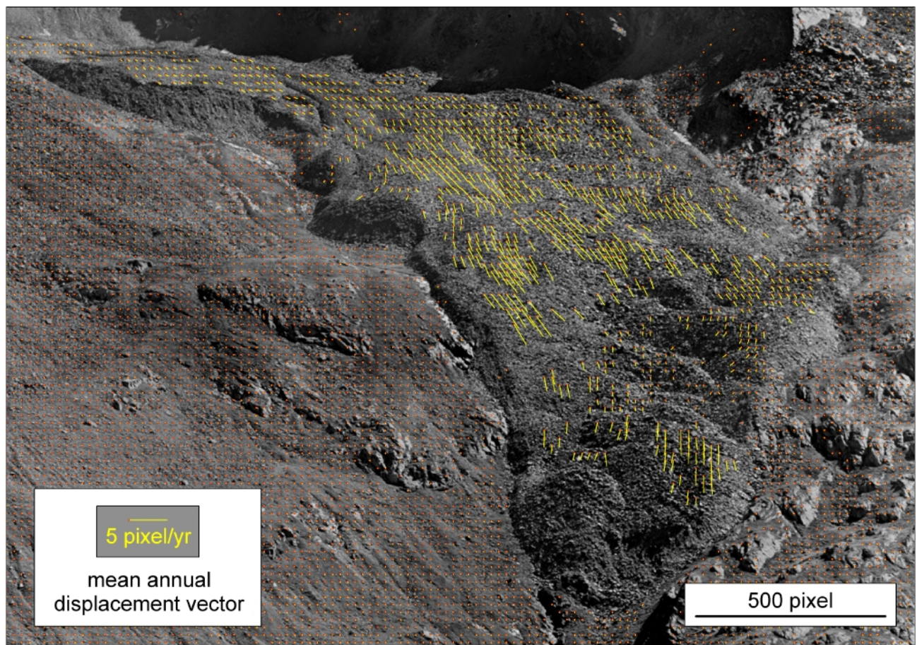
FIGURE 11: This figure shows the 2D vector field (in yellow) of mean annual displacement of surface points of Äußeres Hohebenkar rock glacier for the time period 1986-1999. The reference geometry is based on the Nikon D300 digital image of 2008. The measurement accuracy is \pm 0.1 pixel/yr. Maximum displacements amount to 3.2 pixel/yr in the image plane. The pixel size in nature is 21.1 cm (horizontally and vertically) for the lower end of the rock glacier, 24.6 cm for the central part of the rock glacier, and 33.3 cm for the rooting zone and head walls. The respective ground sampling distances (GSD) are much larger and depend on the inclination of the slope (cp. numerical values given in Ladstädter and Kaufmann, 2004).
