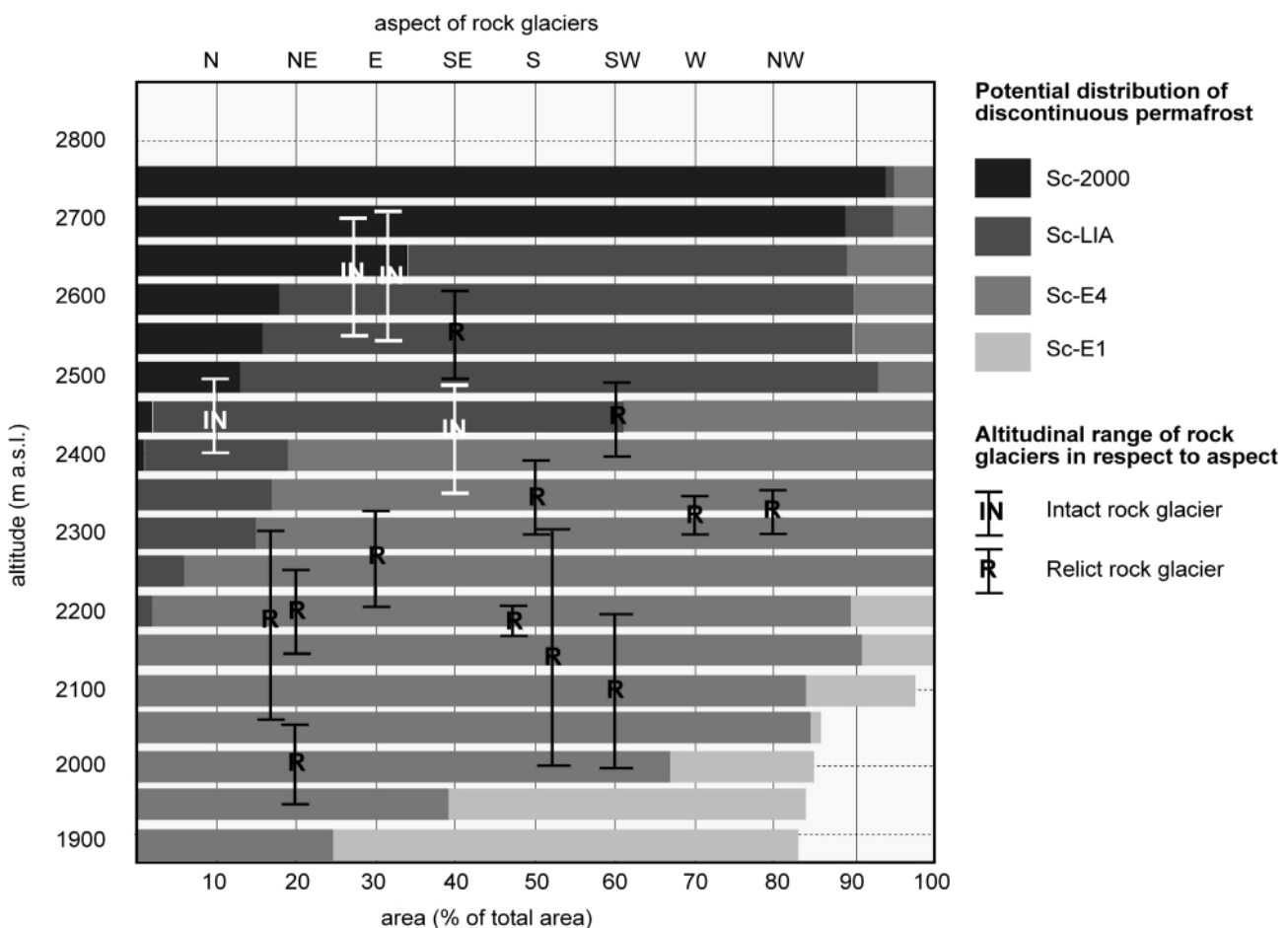
FIGURE 4: Results of four scenarios of modelling potential permafrost distribution in the study area HEG with respect to altitudinal belts (of 50 m steps) as well as altitudinal range of rock glacier range with respect to their activity status.
