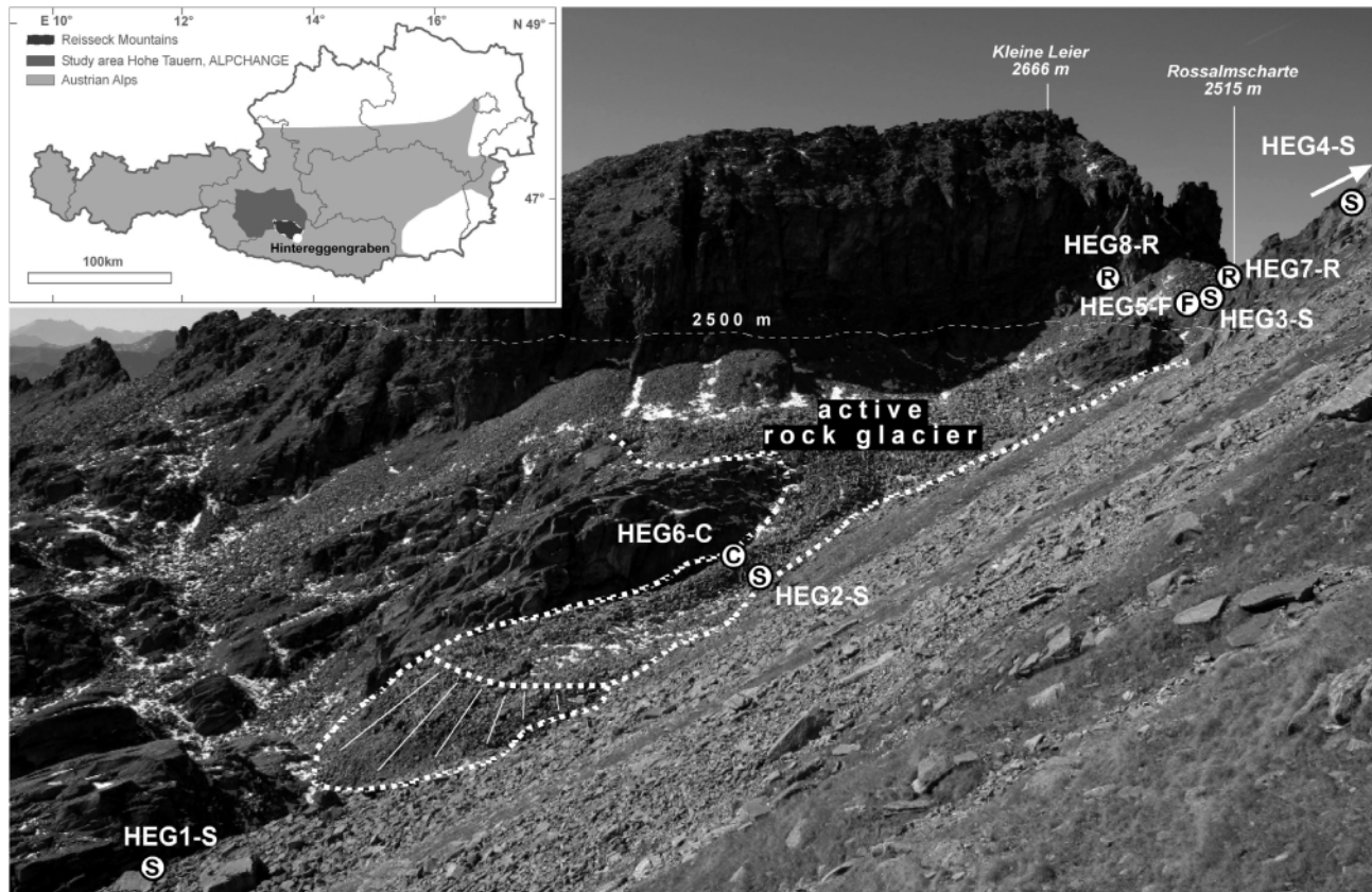
FIGURE 1: The valley head of study area Hinteregggen Valley- Hohe Leier (HEG) showing main landforms and temperature sensor sites with respect to surface conditions: S=surface measurement site; C=coarse-debris site, F=fine-grained site; R=rock wall site. Dotted line indicates margin of the rock glacier. Insert maps shows location of the project area of the ALPCHANGE project within Austria, the study region Reisseck Mountains as well as the local study area HEG.
