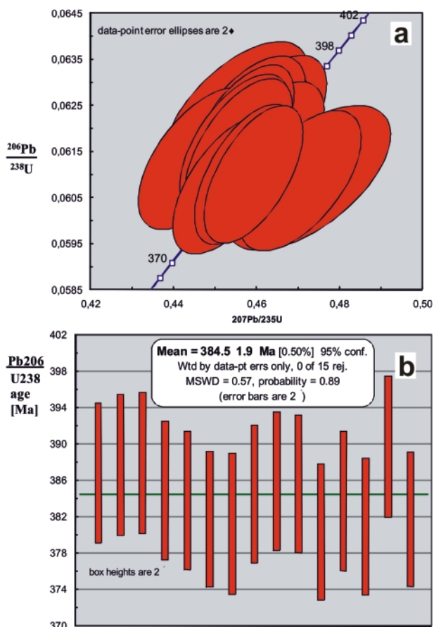
FIGURE 6: a - U-Pb concordia diagram for zircons from a greenschist lens within calcareous phyllites of the Hochglockler facies. b - Mean ^{206}\text{Pb}/^{238}\text{U} age of zircons.
