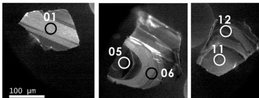
FIGURE 5: Representative cathodoluminescence images of some dated zircons.
