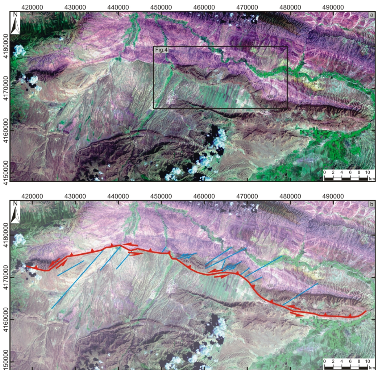
FIGURE 3: a) Aster false color satellite image of the Ashkhaneh Fault (ASHF); the black rectangle is showing the position of Fig. 4. b) transparent version of the Aster false color satellite image overlain by the fault trace of Ashkhaneh Fault (ASHF, red) and the accompanied strike-slip faults (blue); shear sense was only added where measured in the field.
