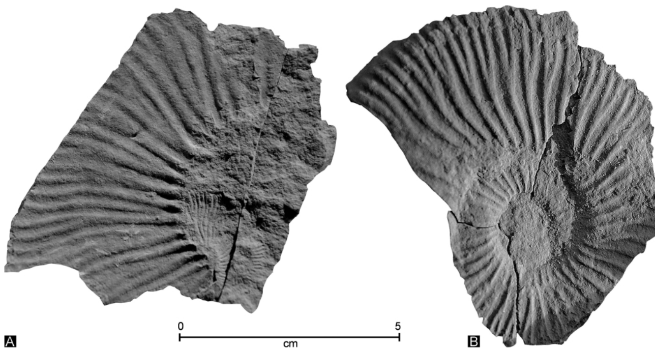
FIGURE 13: Two indicative ammonite fragments (print of the internal moulds) from the investigated section in the Leube open pit. A: Fauriella boissieri (Pictet, 1867), OK-L197. B: Berriasella ( Berriasella ) calisto (d'Orbigny, 1850), OK-L475.
