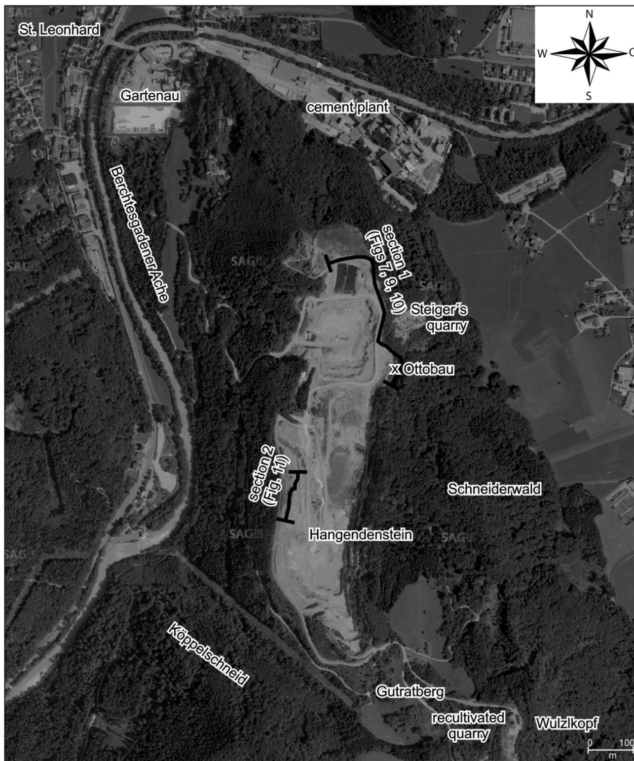
FIGURE 2: Orthophoto (2007-2009) of the Leube open pit mine and the surrounding villages (Geodaten Land Salzburg, Salzburger Geographisches Informationssystem SAGIS, www.salzburg.gv.at/sagis ). The investigated section lines and geographic names mentioned in the text are indicated.
