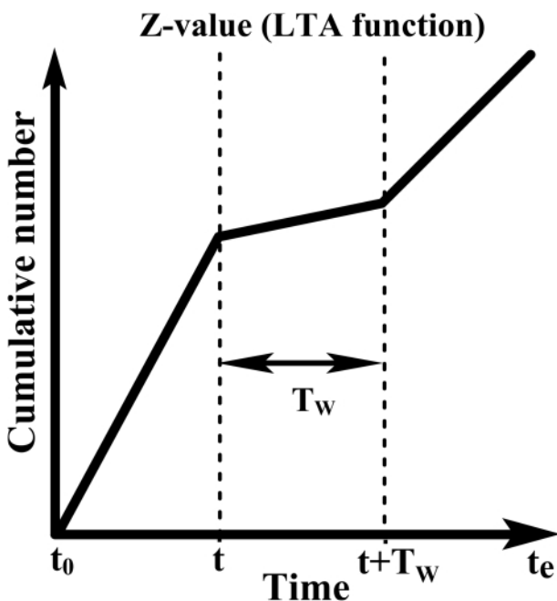
FIGURE 4: Schematic explanation of how to calculate Z-value. The Z-value is calculated for all times t between t_0 and t_e and is statistically appropriate for estimating seismicity rate change in a time window T_w in contrast with background seismicity. T_w is the length of the time window in year and t is the “current time” ( t_0 < t < t_e ).
