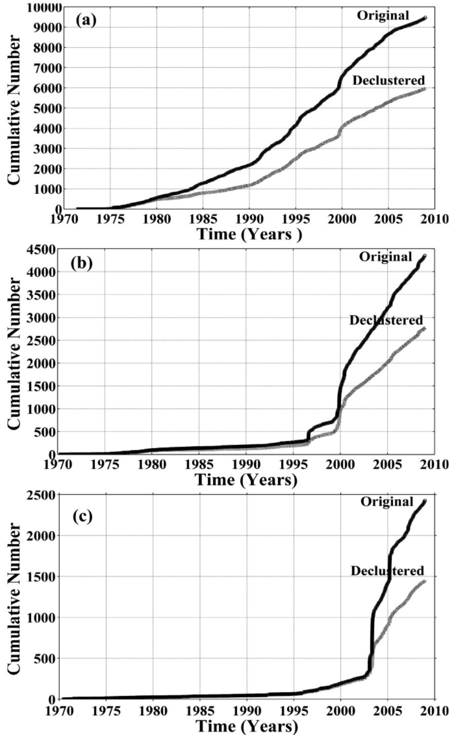
FIGURE 5: Plots of cumulative number of events versus time for original and declustered earthquake catalogues for all sub-regions of the North Anatolian Fault Zone: (a) for MNAFZ, (b) for ANAFZ and (c) for ENAFZ.
