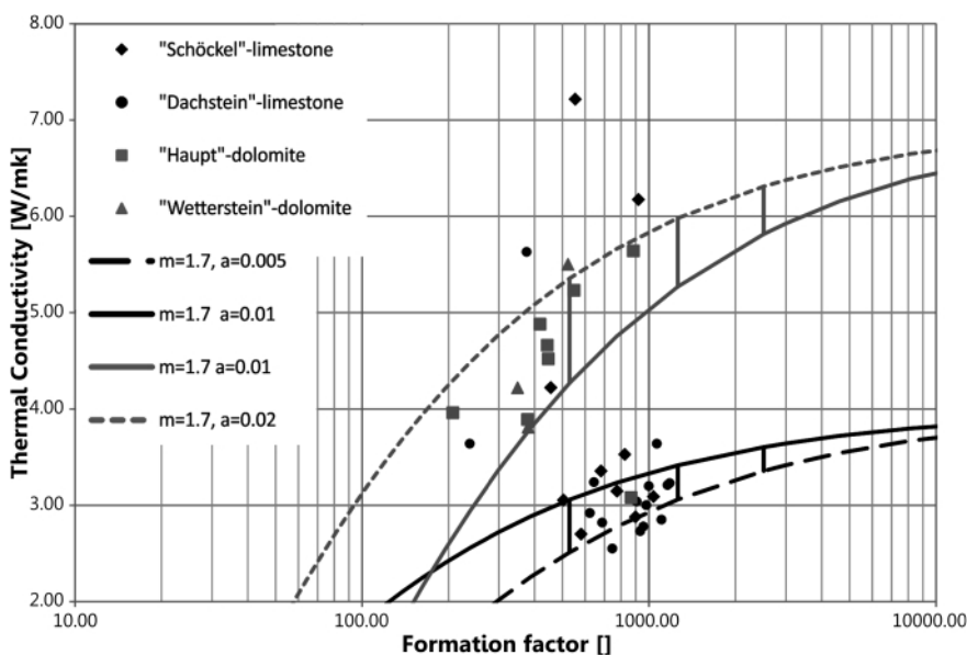
FIGURE 4: Thermal conductivity [ \text{Wm}^{-1}\text{K}^{-1} ] versus formation factor [], lines show calculated results with Archie equation and inclusions model, constant m=1.7 and varying \alpha , grey: dolomite, black: limestone, Connective lines show a porosity of 0.01, 0.02 and 0.03.
