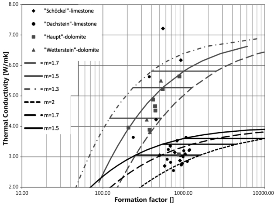
FIGURE 3: Thermal conductivity [ \text{Wm}^{-1}\text{K}^{-1} ] versus formation factor [], lines show calculated results with Archie equation and inclusions model, constant \alpha=0.01 and varying m . Connective lines show a porosity of 0.01, 0.02 and 0.03, grey: dolomite, black: limestone.
