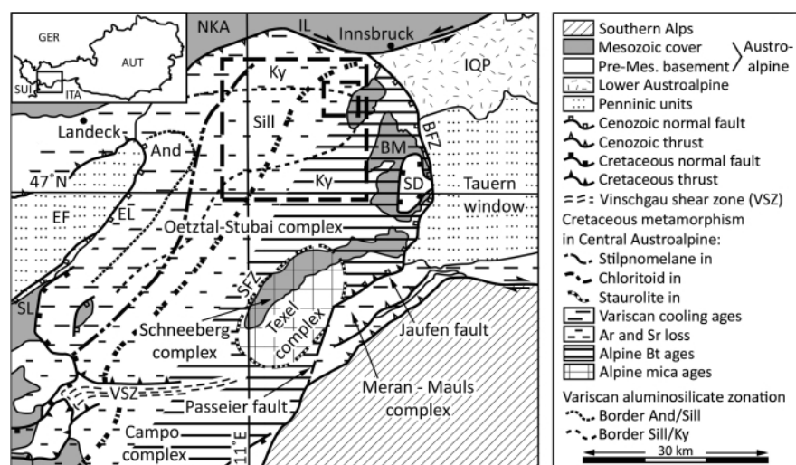
FIGURE 1: Tectonic overview of the Oetztal-Stubai-Complex showing the distribution of Cretaceous metamorphism (redrawn after Fügenschuh et al., 2000), small dashed rectangle: study area, large dashed rectangle: extent of geological map of Hammer (1929). Bfz = Brenner fault zone, BM = Brenner Mesozoic, EF = Engadine window, EL = Engadine line, IL = Inntal line, IQP = Innsbruck Quartzphyllite, NKA = Northern Calcareous Alps, SD = Steinach nappe, SL = Schlingig line, SFZ = Schneeberg fault zone, VSZ = Vinschgau shear zone. Variscan aluminosilicate zonation after Purtscheller (1969): And = Andalusite zone, Ky = Kyanite zone, Sill = Sillimanite zone.
