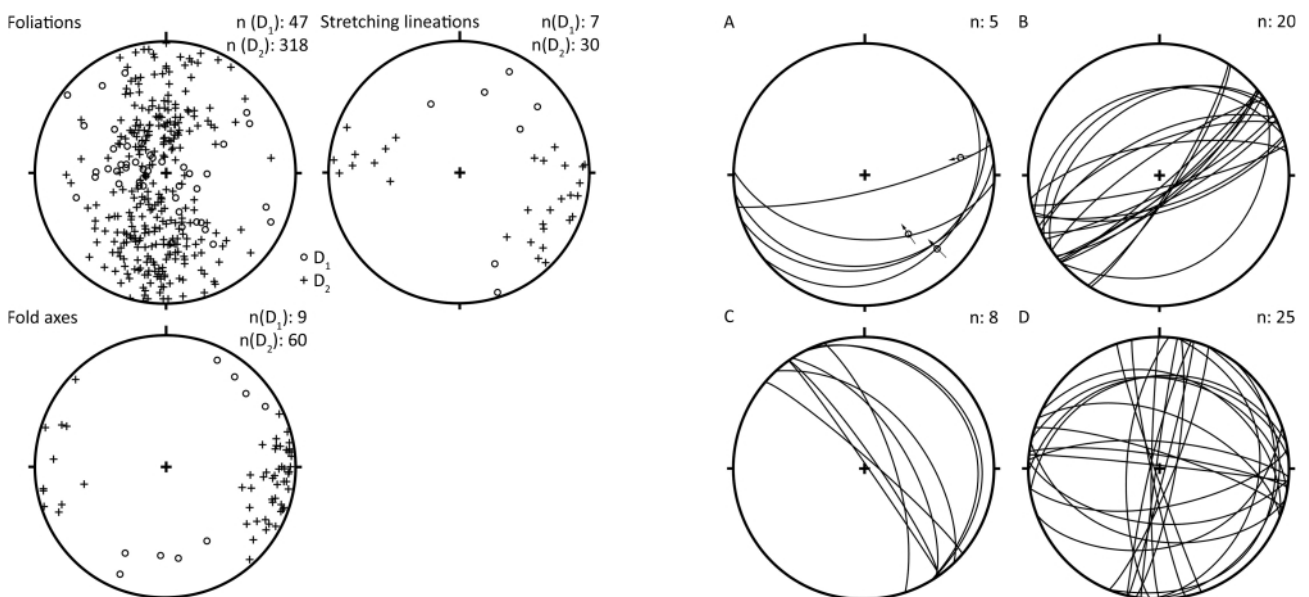
FIGURE 2: Structural data of the investigation area: (left) comparison of D 1 and D 2 foliations, stretching lineations and fold hinges; (right) A: NNW- and W-orientated D 1 thrusts, B: brittle faults related to the Stubaital fault, C: brittle faults related to the Halsl fault, D: brittle faults in the hanging wall of the Brenner fault.
