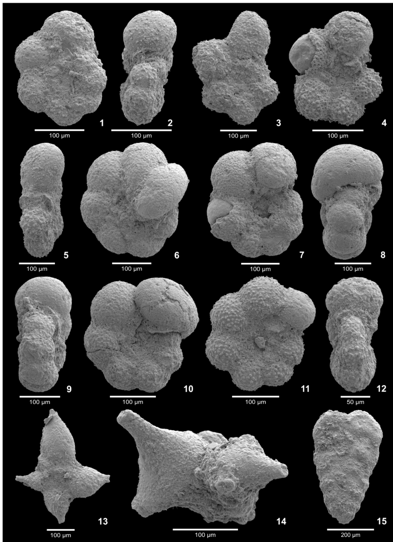
FIGURE 1 1: Scanning electron images of planktonic foraminifera: (1-2) Muricohedbergella planispira (Tappan). (1) spiral view, (2) edge view, (3-5) Hastigerinoides clavatus (Brönnimann). (3) lateral view (slightly trochospiral), (5) edge view, (4) lateral view (planispiral); (6-10) Globigerinelloides bollii Pes-sagno. (6-7) lateral views, (8-9) edge views, (10) lateral view; (11-12) Globigerinelloides ultramicrus (Subbotina). (11) lateral view, (12) edge view; (13) Schackoina cf. cenomana (Schacko). Lateral view; (14) Schackoina multispinata (Cushman and Wickenden); (15) Sigalia deflaensis (Sigal). Frontal view.
