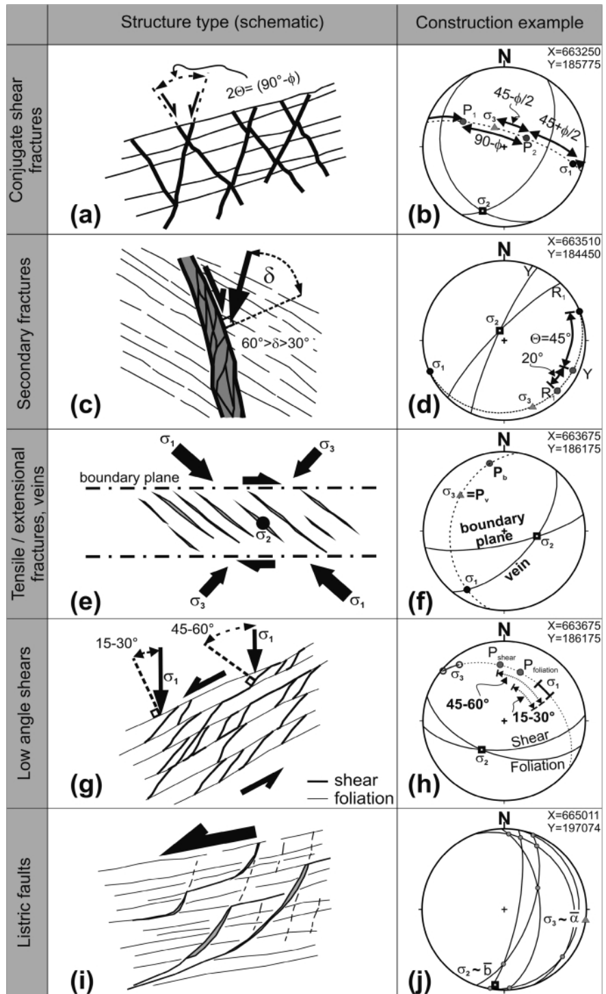
FIGURE 3: Analysed structure types and the respective construction of paleostress axes. (a) Conjugate set of shear fractures with \sigma_1 bisecting the acute angle between the two shear fractures. (b) Construction example for the determination of the paleostress orientations for a given set of conjugate shear fractures (reverse sense of shear, lower hemisphere). (c) Shear zone and related fractures (sinistral sense of shear, see Fig. 5 for nomenclature of fractures). (d) Construction example for the determination of the paleostress orientations for a Y-shear and an associated Riedel shear (strike slip kinematics, dextral sense of shear, lower hemisphere, abbreviations refer to Fig. 5). (e) Vein development and the theoretical orientation of the principal stresses. (f) Construction example for the determination of the paleostress orientations for a given set of veins and the respective boundary plane (lower hemisphere). P_v labels the pole to the vein, P_b the pole to the boundary plane. (g) Low angle shears, bold lines indicate the shear planes, thin lines the metamorphic foliation. (h) Construction example for the determination of the paleostress orientations for low angle shears (lower hemisphere). Only ranges can be given for \sigma_1 and \sigma_3 , P labels the pole to the respective great circle. (i) Listric normal faults. (j) Construction example for the estimation of the azimuth of \sigma_2 and \sigma_3 from listric planes, \sigma_1 is assumed to be vertical. \bar{b} and \bar{a} denote the mean intersection axis and the mean azimuth of the measured planes.
