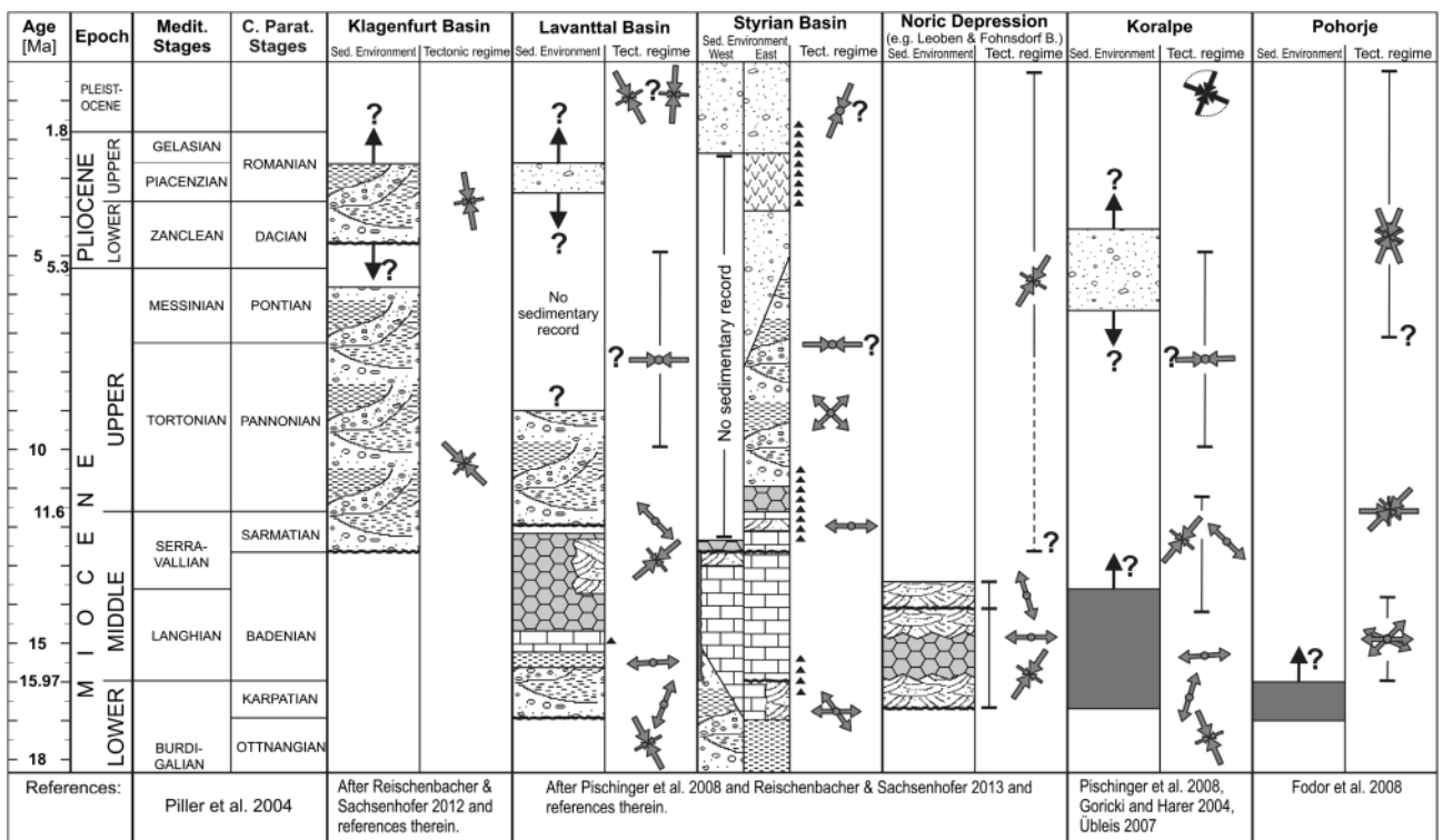
FIGURE 2: Schematic correlation of the sedimentary evolution and the paleostress regime for the Klagenfurt, the Lavanttal and the Styrian Basin, as well as for the Noric Depression, the Koralpe and the Pohorje from the Ottnangian (Lower Miocene) to Pleistocene.
