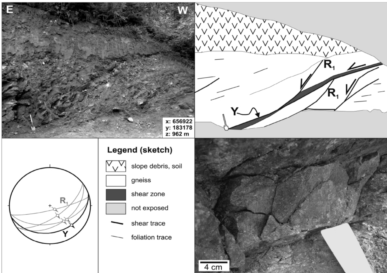
FIGURE 6: Faulting related secondary fractures of a cataclastic shear zone with normal sense of shear in gneissic bedrock of the eastern Koralmpe. Y-shear - Riedel shear configuration is observable on the outcrop (spade is approx. 60 cm long) and the hand specimen scale (lower right, picture was taken just left of the upper left photograph). Angelier plot (Equal-area projection, lower hemisphere) shows orientation and sense of shear for the Y-shear (black great circle) and several Riedel shears.
