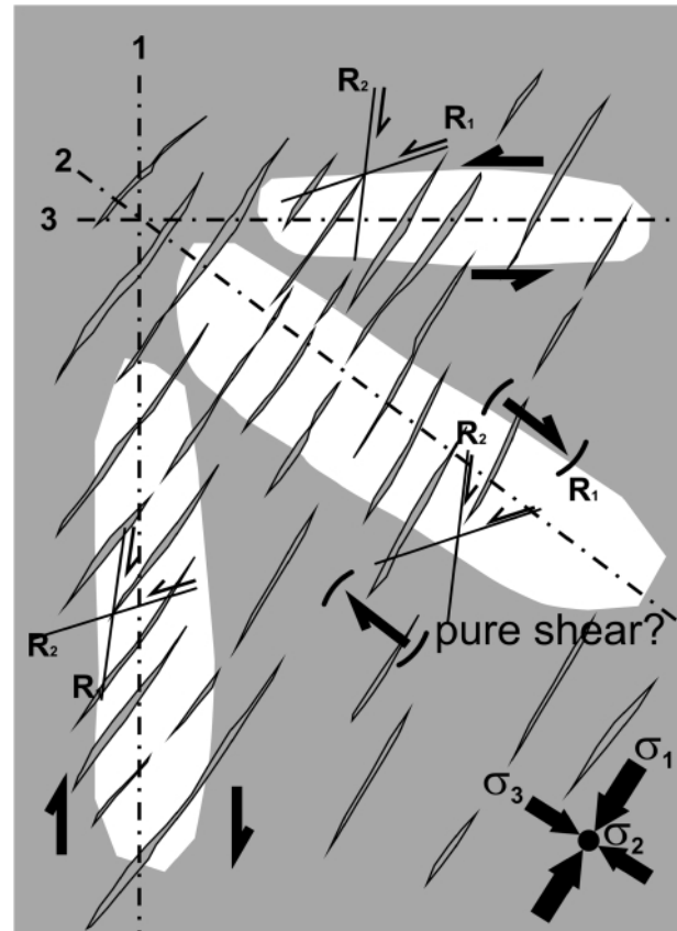
FIGURE 16: Schematic system of extension veins with \sigma_1 parallel and \sigma_3 at right angles to the depicted vein traces. Axis of \sigma_2 is perpendicular to the plane of the sketch (see lower right corner of figure). Limited exposure is marked by white patches and, if not considered, may result in a biased determination of shear kinematics from different outcrop orientations (dashed lines 1, 2, 3 and blank fields) and an erroneous interpretation.
