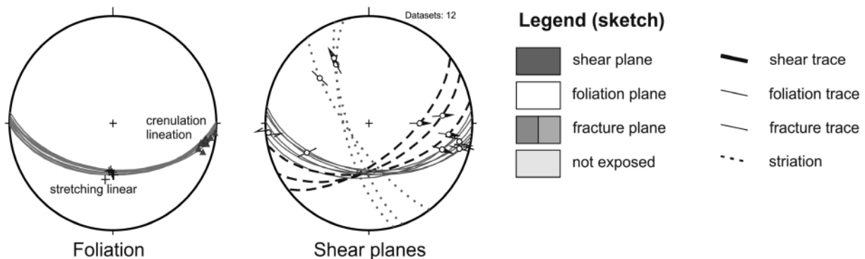
FIGURE 8: Outcrop in "Plattengneis" mylonite of the central Koralpe, exposing low angle shear planes and shearing of foliation. Left Equal-area projection (lower hemisphere) displays foliation with stretching (crosses) and crenulation lineation (triangles). Right diagram (Angelier plot) shows low angle shears (dashed great circles), slightly steeper than foliation parallel shears (continuous great circles). Steep WSW dipping shear planes (dotted lines) are not visible in the photograph. In this location striations indicate strike-slip displacement. Striations plot in similar direction as crenulation lineation, but are clearly distinguishable from the crenulation lineation.
