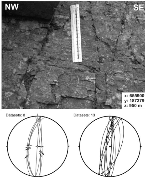
FIGURE 4: Outcrop in "Plattengneis" mylonite, exposing conjugate shear planes with (Angelier plot, left side) and without striation (right plot). Conjugate shears with striations constrain W-E directed extension of shears without striation. Note eastward displacement along foliation parallel shear plane below the scale bar. Equal-area projection, lower hemisphere. Scale in photograph is 15 cm.
