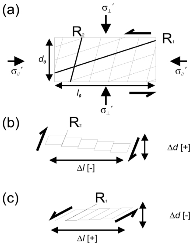
FIGURE 7: Initial shear zone development, where the formation of R_1 and R_2 is equally probable: (a) Geometry for the development of initial shear planes, (b) comparatively high \sigma_3' leading to preferred development of R_2 , (c) comparatively low \sigma_3' causing the development of R_1 . SZB; Y- and P- shear elements have not yet developed for the depicted stages ( l_0 ...initial length, d_0 ... initial thickness).
