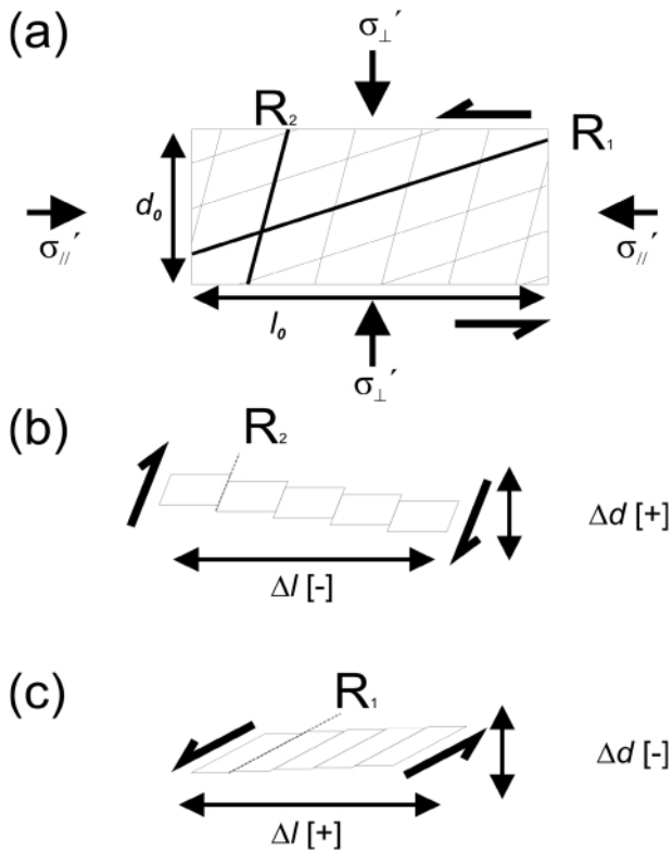
FIGURE 7: Initial shear zone development, where the formation of R_1 and R_2 is equally probable: (a) Geometry for the development of initial shear planes, (b) comparatively high \sigma_3/\sigma_1 leading to preferred development of R_2 , (c) comparatively low \sigma_3/\sigma_1 causing the development of R_1 . SZB; Y- and P- shear elements have not yet developed for the depicted stages ( l_0 ...initial length, d_0 ... initial thickness).
