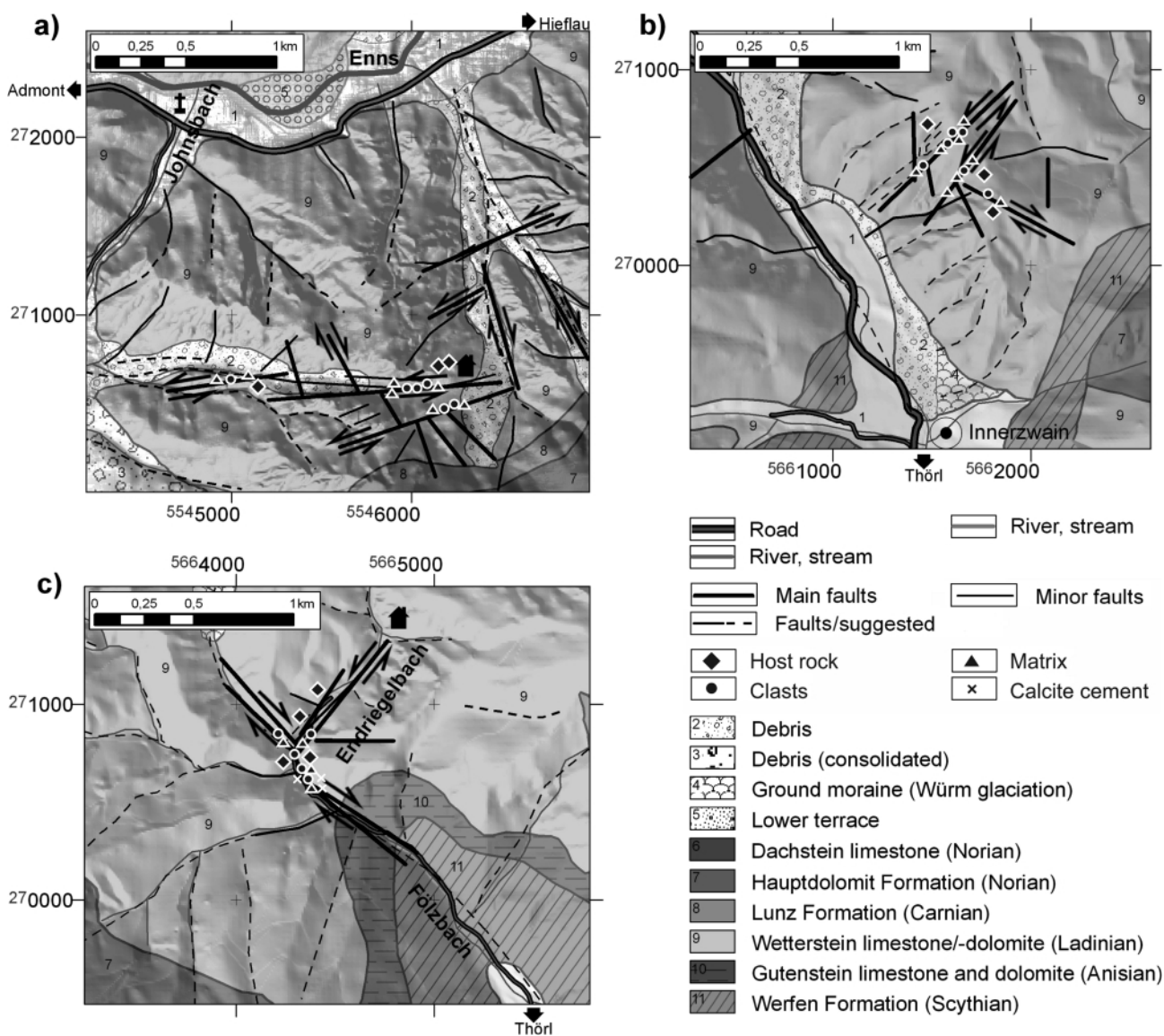
FIGURE 2: Digital Terrain Model (DTM) with overlaying geological map and sample locations of (a) site Haindlkar, (b) site Brandwald and (c) site Fölz (modified after Hausegger and Kurz 2013). Indication of sample locations (Tab.1) is sub-divided in „host rock“, „clasts“, „matrix“ and „cement“-samples. Only fault zones that were identified in the field are displayed.
