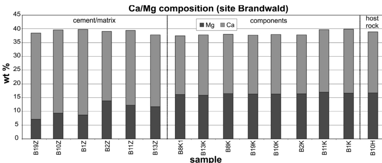
FIGURE 15: Ca and Mg composition of powder samples from site Brandwald. While the Ca/Mg ratio is constant in host rock and cataclasite clasts, matrix samples exhibit distinct indications for de-dolomitization, illustrated by a distinct change of Ca/Mg ratio (decreased Mg- and increased Ca content).
