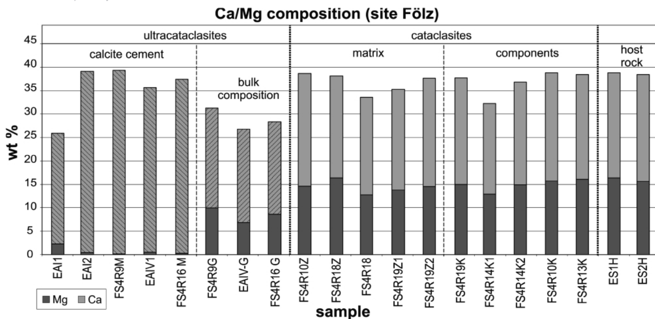
FIGURE 16: Ca and Mg composition of powder samples from site Fölz. Ca/Mg ratios of host rock and cataclasite samples exhibit only slight variations. However, ultracataclasite matrix show very low Mg contents and indicate distinct evidence of almost complete de-dolomitization of matrix material into calcite.
