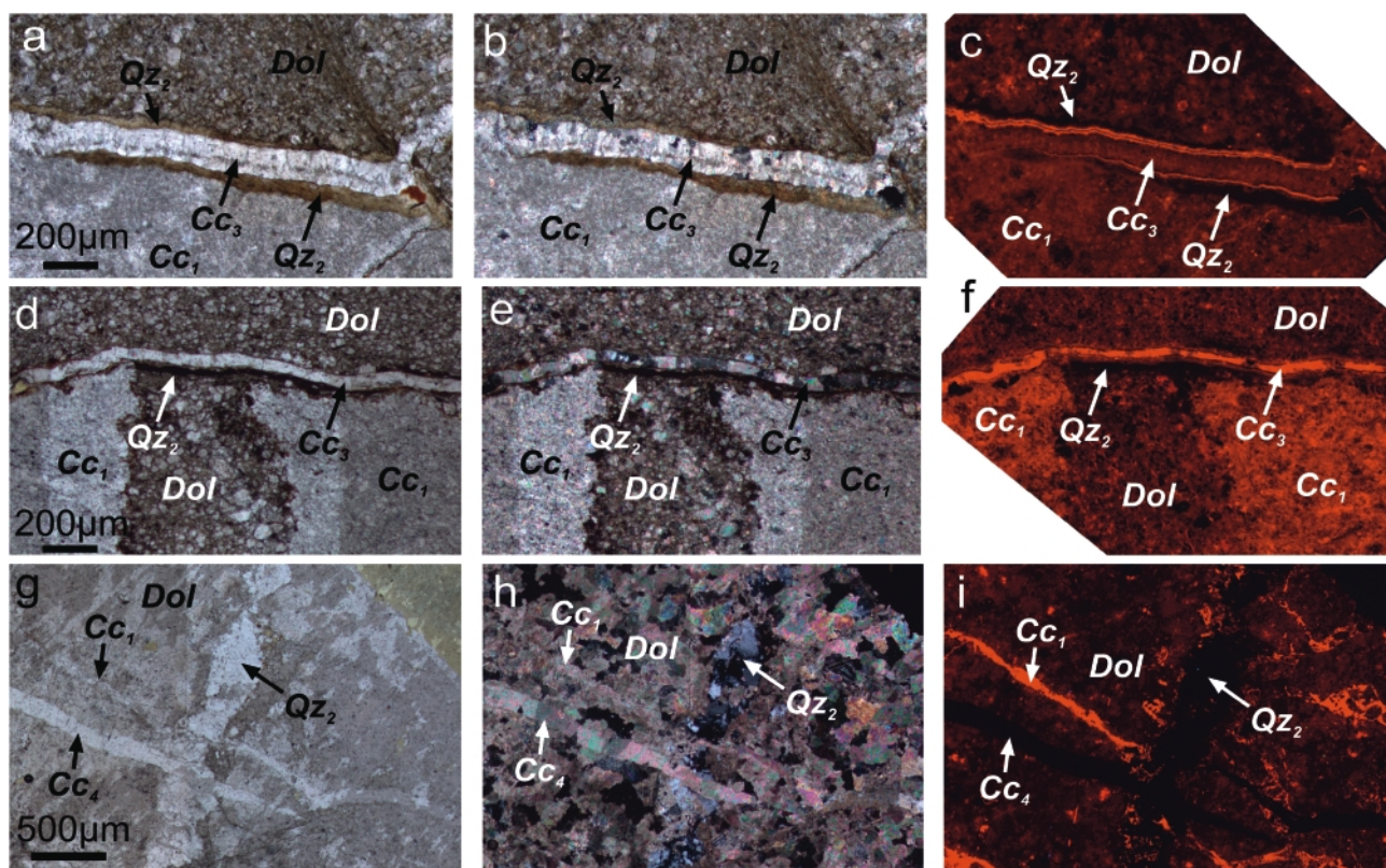
FIGURE 8: (a, d) Plane-light, (b, e) cross-polarized light and (c, f) CL image of an ultracataclastite from site Fölz (samples EA1, EA2). (g) Plane-light, (h) cross-polarized light and (i) CL image of a fault core cataclastite from site Fölz (sample R14). Parent rock material is dolomite ('Dol'). Dedolomitized material and vein fillings ('Cc 1 '), quartz filled veins ('Qz 2 ') and subsequent calcite veins ('Cc 3 and Cc 4 ') are distinguished.
