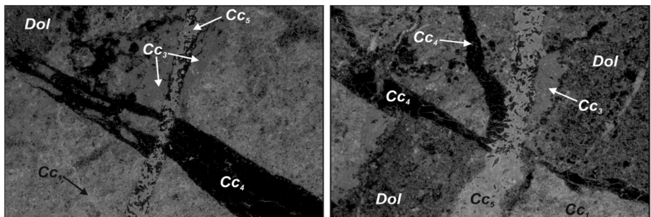
FIGURE 11: CL images of ultracataclasites from site Fözl (samples EA1 and EA2) illustrating CL behavior and chronological sequence of all five precipitation phases (phase P1 to P5). Calcite cement derived from de-dolomitization ('Cc 1 ') and phase P3 ('Cc 3 ') show intermediate to bright luminescence. Calcite veins from phase P4 ('Cc 4 ') with no luminescence developed sub-perpendicular to Cc 3 -veins. Bright red calcite veins from phase P5 ('Cc 5 ') strike through dark Cc 4 veins, dragging non-luminescent material from phase P4 along the course of P5 veins.
