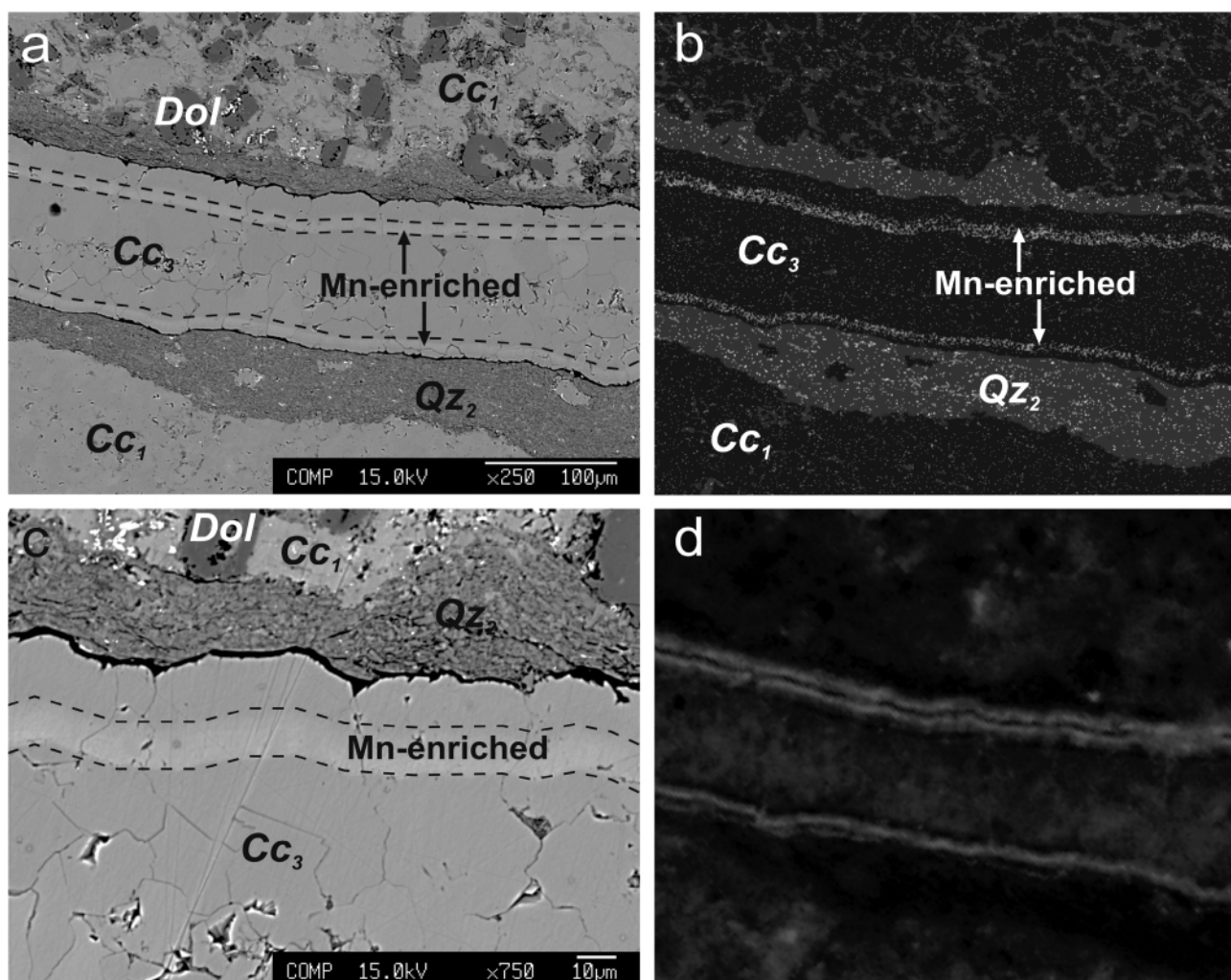
FIGURE 10: (a, c) BSE image of a secondary calcite vein in ultracataclasite sample EA1. Dolomite clasts ('Dol') are embedded in de-dolomitized material ('Cc 1 '). Calcite vein Cc 3 strikes through former quartz veins ('Qz 2 ') and exhibits internal zonation, showing bands of increased Mn content. (b) Combined element mapping of Si, Mn and Fe illustrates Mn enriched bands and quartz precipitation in veins and intergranular pore space. (c) Detailed image of the upper rim of the calcite vein. (d) CL image clearly illustrates the bright luminescence of Mn-enriched bands. Dedolomite domains show darker luminescence colours. Quartz rich areas stay dark.
