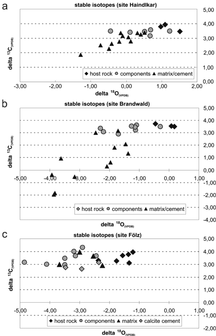
FIGURE 12: Stable isotope compositions ( \delta^{13}\text{C} and \delta^{18}\text{O} in ‰) of host rock slices as well as cataclasite clasts, cataclasite matrix and secondary calcite cement from fault core samples from (a) site Haindlkar, (b) site Brandwald and (c) site Fölz. All sites indicate the tendency of decreased \delta^{18}\text{O} values in the course of evolution from host rock to cataclasite components and matrix/cement. (a, b) Dedolomitized matrix material from site Haindlkar and Brandwald show decreased \delta^{13}\text{C} values.
