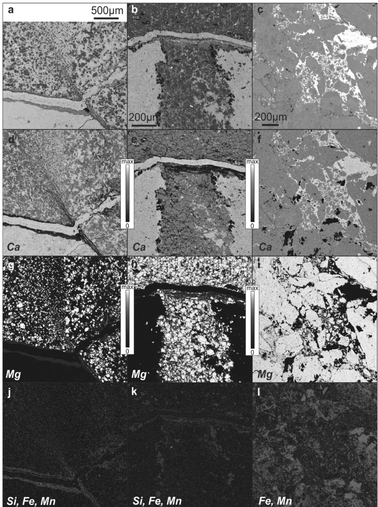
FIGURE 9: BSE image of (a, b) ultracataclasite (samples EA1 and EA2) and (c) fault core cataclasites (sample R14). Calcite (Ca) is shown in bright grey to white and dolomite (Mg) in dark grey colors. (d-f) Mapping of Ca content. (g-i) Mapping of Mg content. (j, k) Compiled element mapping of Si, Fe and Mn of ultracataclasite samples EA1 and EA2 showing constant Mn distribution (dark) and increased Fe- (gray) and Si- (bright grey) content in the outer rims of calcite filled veins and in intergranular pore volume. (l) Compiled Fe-Mn mapping of cataclasite sample R14. Mn shows constant distribution, whereas Fe content in calcite areas is very low. All samples from site Fölz.
