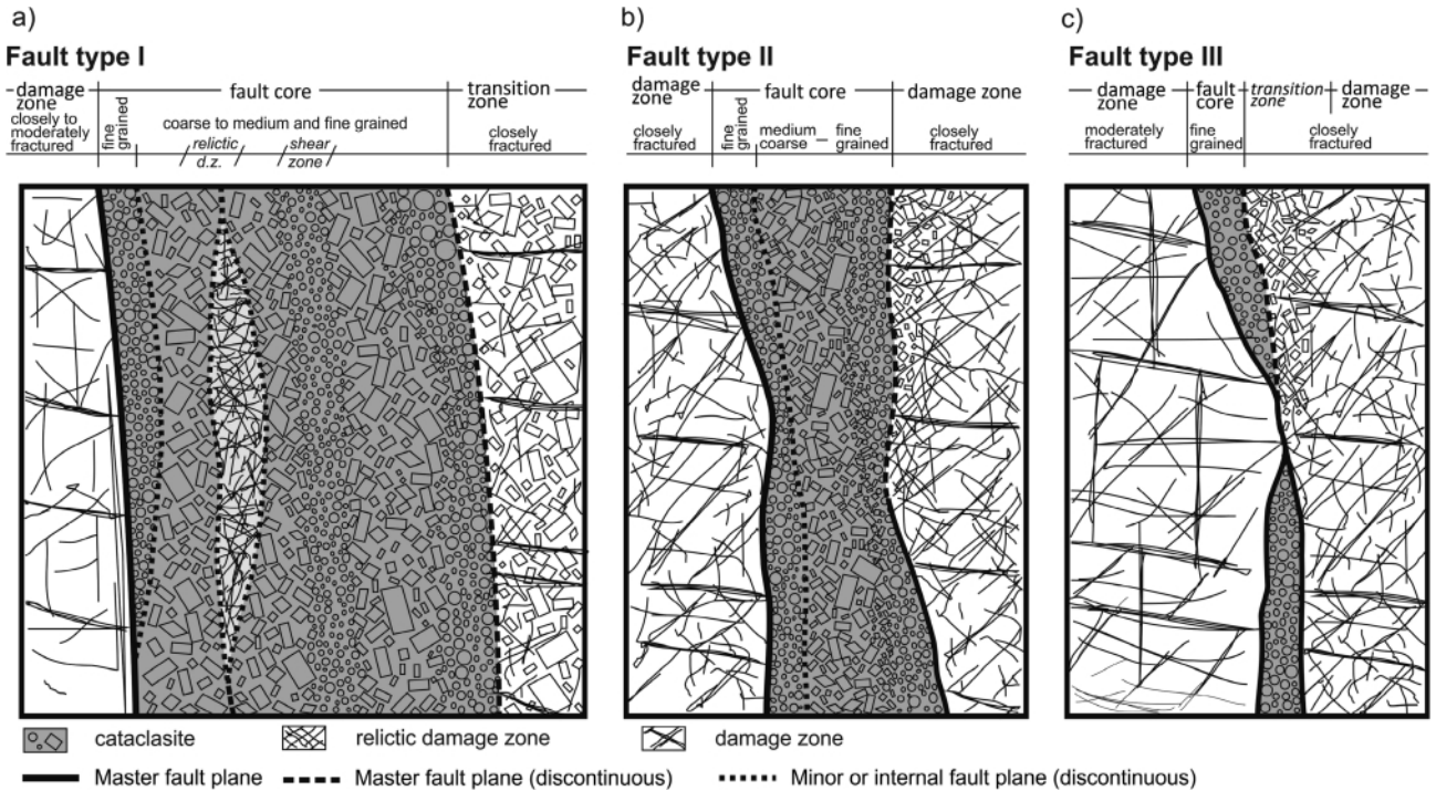
FIGURE 3: Conceptual cross sections of classified fault types (modified after Hausegger and Kurz 2013). (a) Fault type I (exclusively in main fault orientation and suitable thickness of more than 1m) is characterized by a complex internal fault core structure, composed of several domains of cataclasites, host rock lenses and internal fault planes (slickensides). (b) Fault type II shows an advanced state of fault core segmentation (shear bands and internal fault planes/slickensides) and thickness from 20 to 100 cm. (c) Fault type III is classified as uniform and solitary cataclasite layer with thicknesses less than 20 cm. All fault core cataclasites are composed of comminuted fragments (clasts) in a very fine-grained matrix of pulverized host rock (dolomite) and variable amount of secondary calcite.
