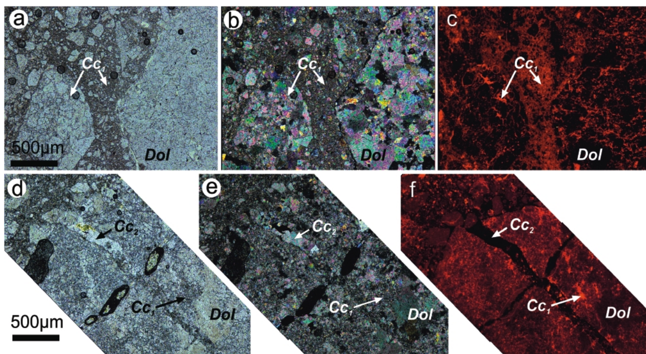
FIGURE 6: (a) Plane-light, (b) cross-polarized light and (c) CL image of a fault core cataclasite from site Brandwald (fault type II; sample B8). (d) Plane-light, (e) cross-polarized light and (f) CL image of the main fault core cataclasite from site Brandwald (fault type I; sample B11). Parent rock material is dolomite ('Dol') with secondary calcite fillings, dedolomitized crystal rims and matrix material ('Cc 1 ') as well as subsequent calcite veins ('Cc 2 ').
