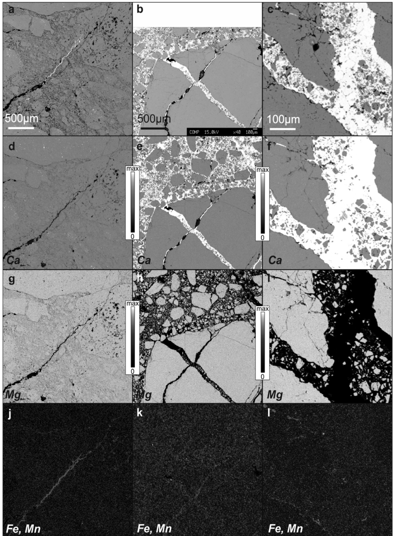
FIGURE 7: BSE image of (a) fault core cataclasite (fault type II; sample B8), (b) fault core cataclasite (fault type I; sample B11) and (c) detailed image of a calcite vein in fault type I cataclasites. Calcite and Fe-rich vein fillings (a) are shown in bright grey to white and dolomite in dark grey colors. (d-f) Mapping of Ca content. (g-i) Mapping of Mg content. (j-l) Compiled Fe-Mn mappings express areas of increased Fe-content (brighter areas and veins). All samples from site Brandwald.
