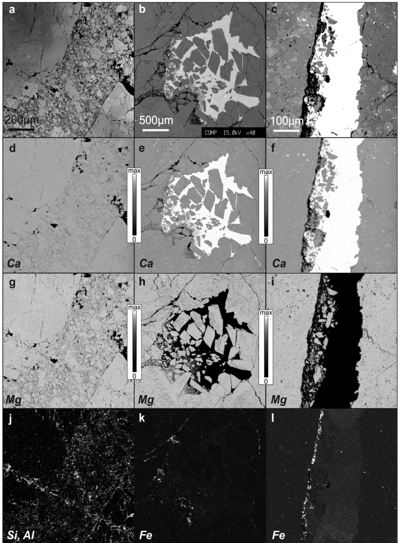
FIGURE 5: BSE image of (a) fault core cataclasite (sample G7), (b) damage zone (sample H4) and (c) detailed image of a damage zone calcite vein. In BSE images calcite is shown in bright grey to white and dolomite in dark grey colors. (d-f) Mapping of Ca content. (g-i) Mapping of Mg content. (j) Compiled element mapping of Si and Al of sample G7 (fault core cataclasite). (k, l) Fe mapping of sample H4 (damage zone) showing slightly increased Fe contents which quenches CL in areas of secondary calcite. All samples from site Haindlkar.
