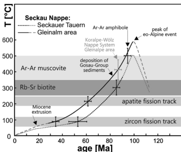
FIGURE 7: T-t paths for the different parts of the Seckau Nappe: Prior to the Eo-Alpine metamorphic peak the Seckau Complex and the overlying Permian-Triassic sediments were heated. The Eo-Alpine metamorphic peak was reached at 90–100 Ma. Rocks from the Seckauer Tauern experienced lower peak conditions as those in the Gleinalm area (about 500 °C) and cooled earlier than the latter. Diagram based on data from Dunkl et al. (2005), Faryad and Hoinkes (2001, 2003), Hejl (1997), Neubauer et al. (1995) and Scharbert (1981). Greyish lines indicate expected parts of T-t path. For explanation see text.
