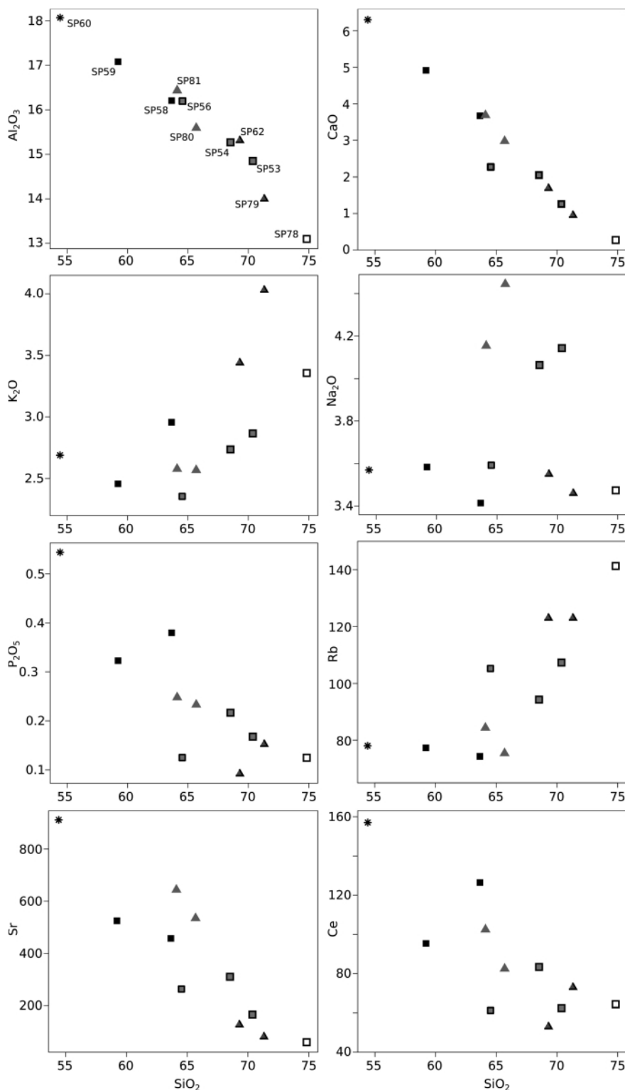
FIGURE 3: Harker diagrams with selected major and trace elements. The porphyritic samples (black squares) have low \text{SiO}_2 values but are high in \text{CaO} , \text{P}_2\text{O}_5 , \text{Sr} and \text{Ce} . The S-type orthogneiss samples SP62 and SP79 (gray triangles with black outline) are relatively enriched in \text{SiO}_2 , \text{K}_2\text{O} and \text{Rb} , while low in \text{CaO} , \text{Na}_2\text{O} , \text{P}_2\text{O}_5 , \text{Sr} and \text{Ce} .
