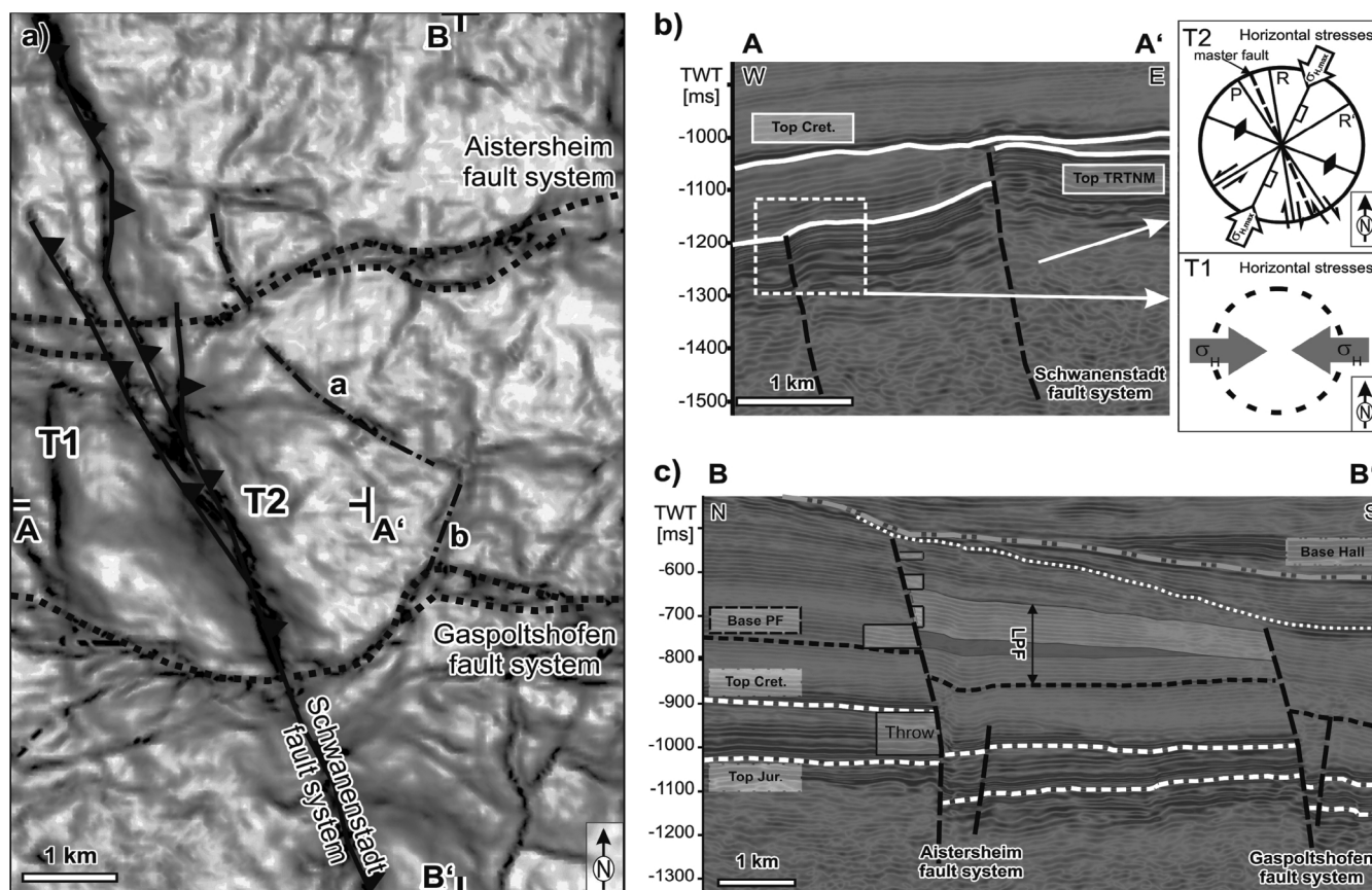
Figure 10: a) Relief map of Top Cenomanian. A-A' and B-B' represent profiles shown in b) and c). b) Mesozoic faults and associated horizontal stresses. c) Cenozoic faults. Note that throws increase downwards (LPK = Lower Puchkirchen Fm.).
