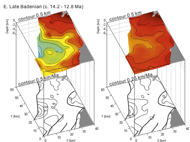
Figure 11: 3D subsidence depth (above) and subsidence rate (below) maps of the basement subsidence (left) and tectonic subsidence (right) visualized in the study area; D: early Badenian (c. 16.3 – 14.2 Ma) and E: late Badenian (c. 14.2 – 12.8 Ma). The major faults are shown with black solid lines in the rate map.
