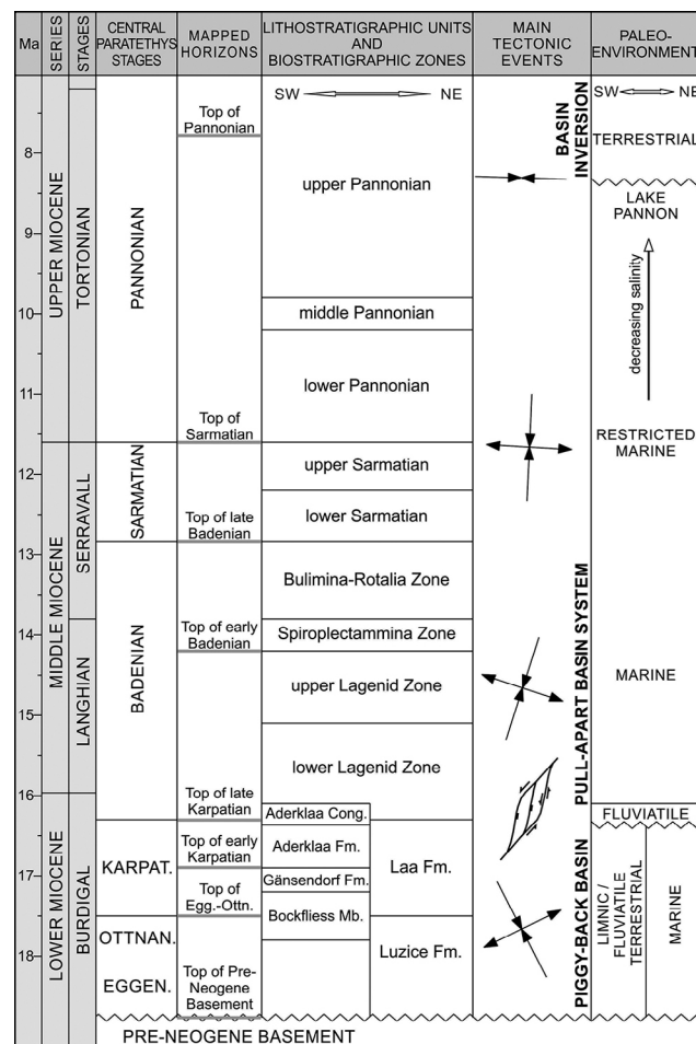
Figure 2: Stratigraphy and evolution of the Vienna Basin in the Miocene (Decker, 1996; Fodor, 1995; Hohenegger et al., 2014; Hölzel et al., 2010; Peresson and Decker, 1997a; Piller et al., 2007; Wagreich and Schmid, 2002). Horizons mapped in this study are; top of the Pre-Neogene Basement, top of the Eggenburgian-Ottangian, top of the early Karpatian, top of the late Karpatian, top of the early Badenian, top of the late Badenian, top of the Sarmatian, and top of the Pannonian.
