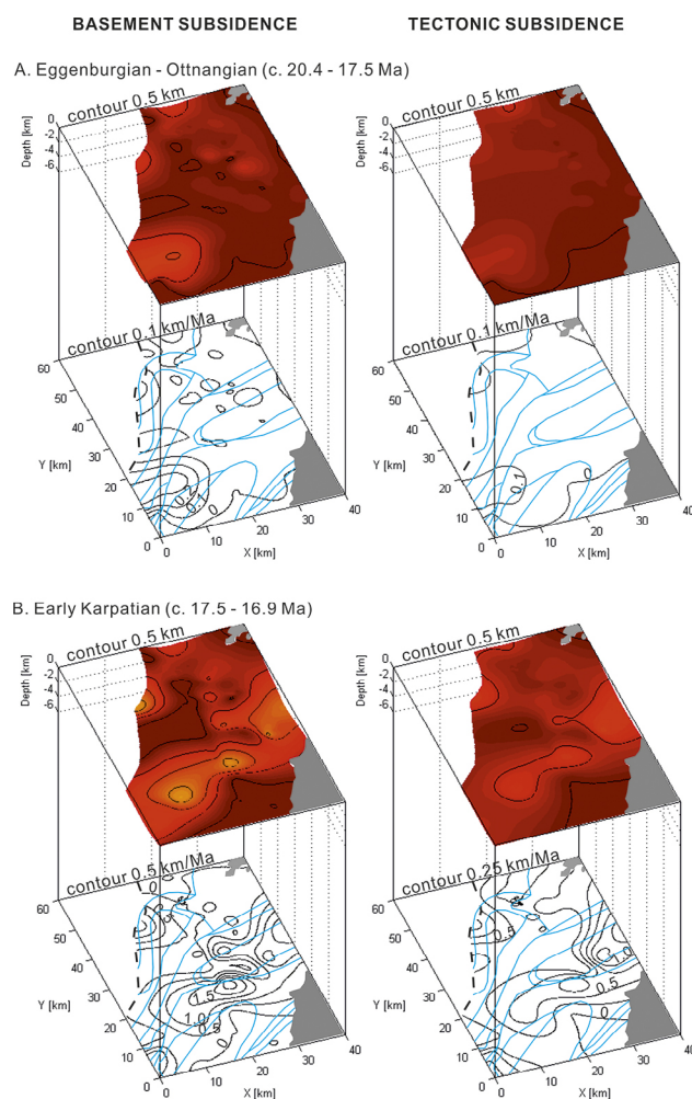
Figure 9: 3D subsidence depth (above) and subsidence rate (below) maps of the basement subsidence (left) and tectonic subsidence (right) visualized in the study area; A: Eggenburgian–Ottangian (c. 20.4 – 17.5 Ma) and B: early Karpatian (17.5 – 16.9 Ma). The Alpine–Carpathian thrust nappe borders are shown with blue solid lines and the location of the Steinberg fault with black broken lines.
