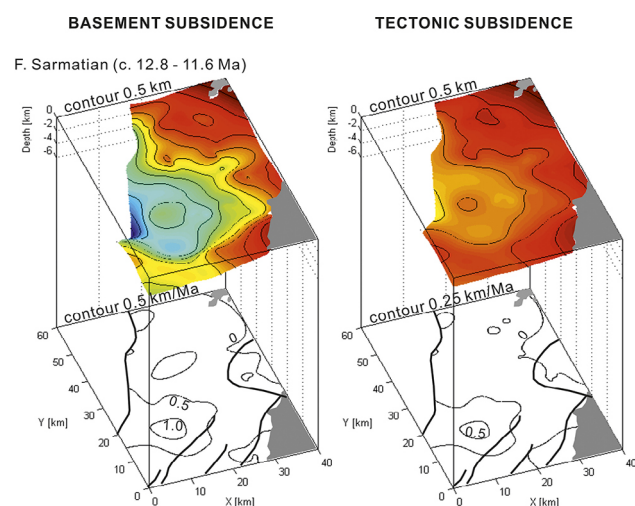
Figure 12: 3D subsidence depth (above) and subsidence rate (below) maps of the basement subsidence (left) and tectonic subsidence (right) visualized in the study area; F: Sarmatian (c. 12.8 – 11.6 Ma) and G: Pannonian (c. 11.6 – 7.8 Ma). The major faults are shown with black solid lines in the rate map.
