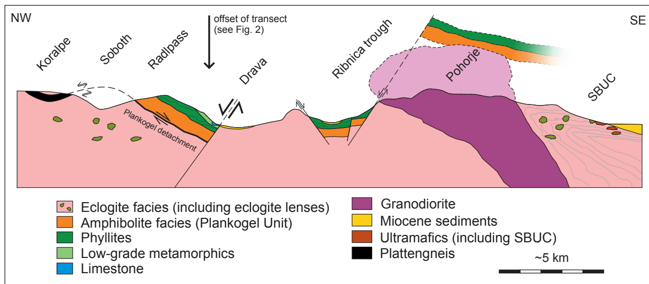
Figure 7: Geological profile through the studied transect as inferred from our metamorphic data and consistent with Fig. 2. The sense of shear for the Plankogel detachment and the Plattengneis are after Schorn and Stüwe (2016). The normal faults near the Drava valley and the Ribnica trough are inferred to be consistent with normal faulting during the 2 nd stage of exhumation as suggested by Neubauer (1995) and as seen on the map on Fig. 1. The arrow indicates the location of the jump in the section.
